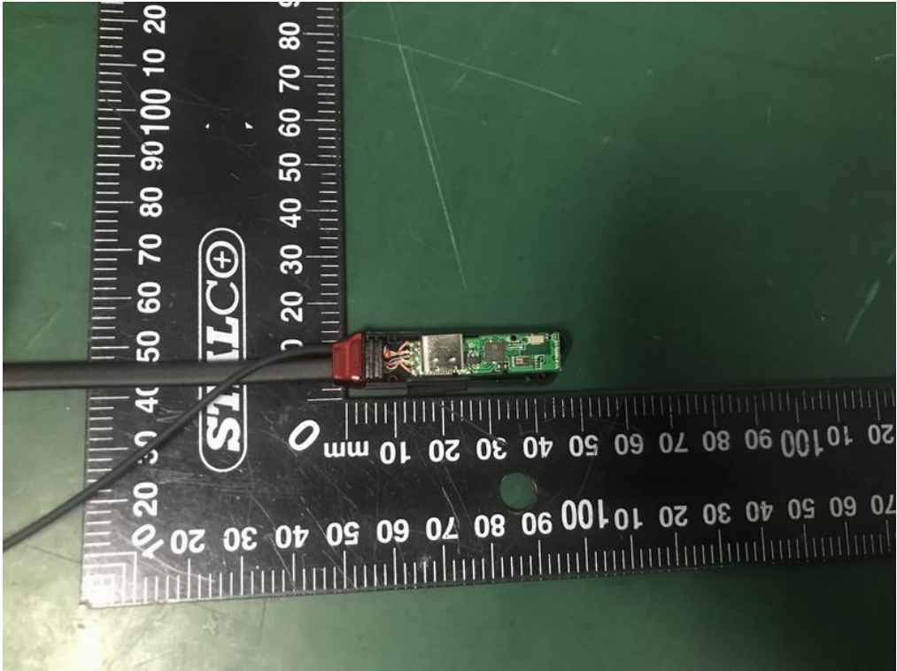
Internal Photos M/N: MH11906
