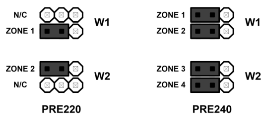
Jumper settings for enabled talkover
