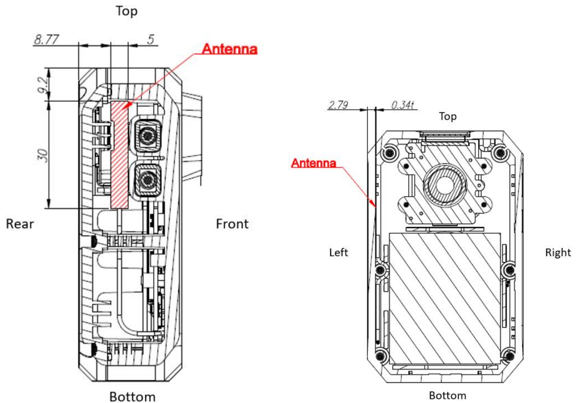
Figure E-1 Antenna Location
