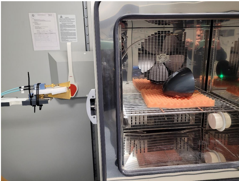
Photo 11 Test Setup frequency stability
