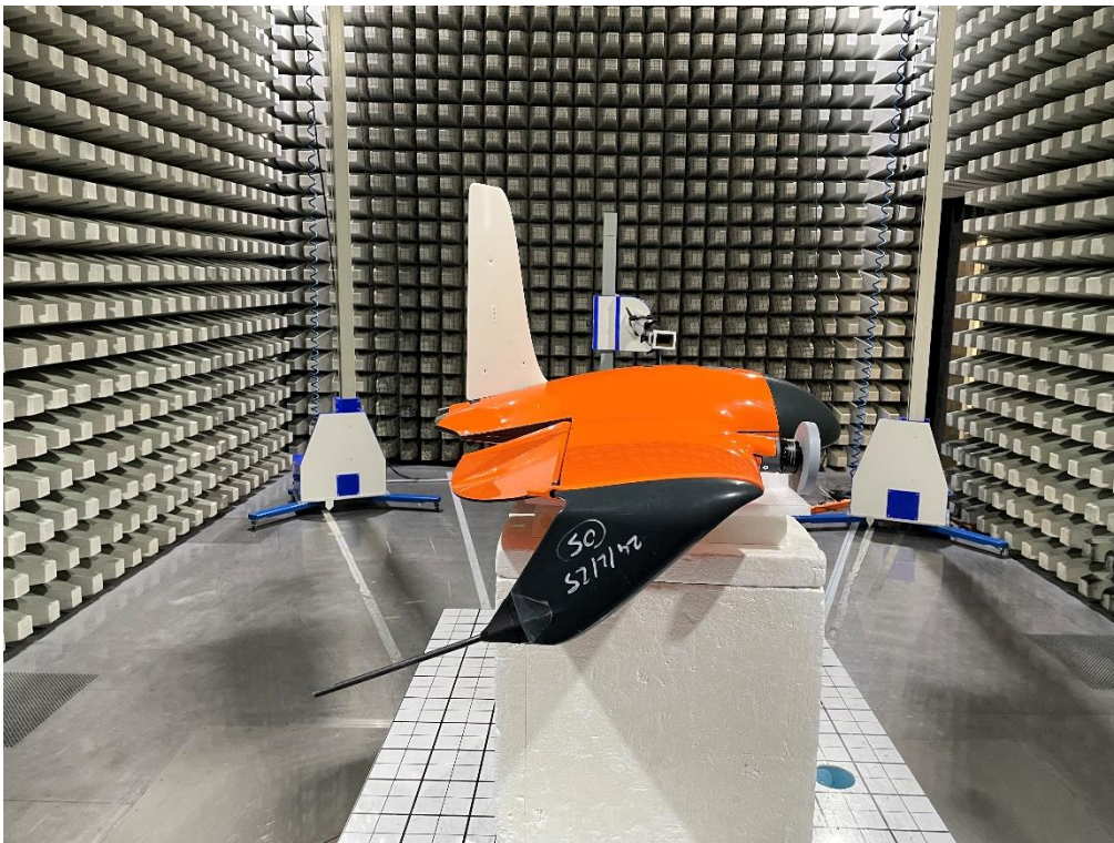
Photo 8 Radiated Test Setup 18-40 GHz
