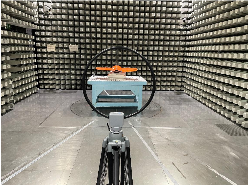
Photo 1 Radiated Test Setup below 30 MHz
