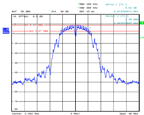
(802.11b) 6dB Bandwidth plot on channel 11
