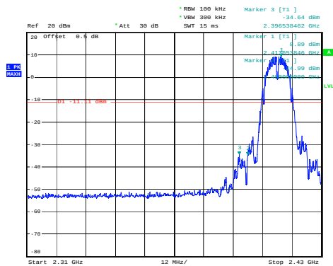
802.11b: Band Edge-Low Channel
