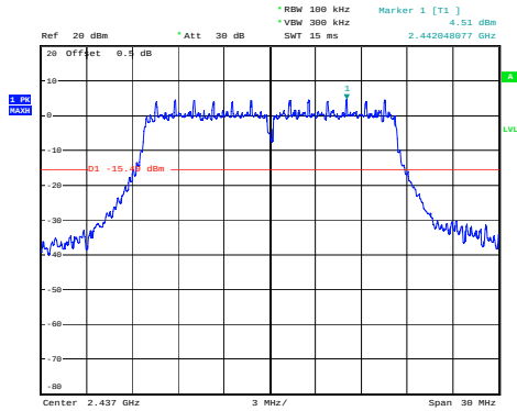
802.11g on channel 06
