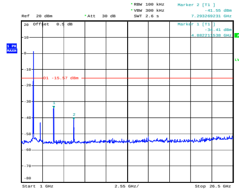
802.11 n20 on channel 06
