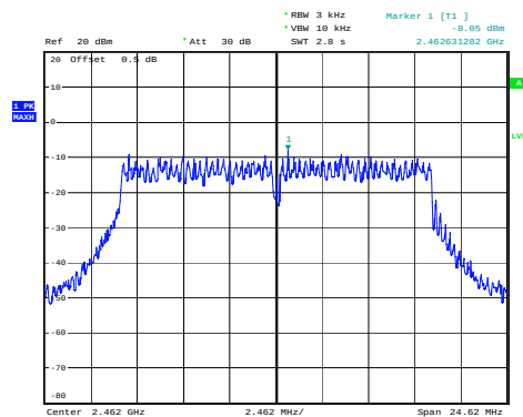
(802.11g) PSD plot on channel 11
