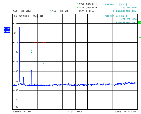
802.11b on channel 01
