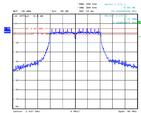
(802.11g) 6dB Bandwidth plot on channel 6
