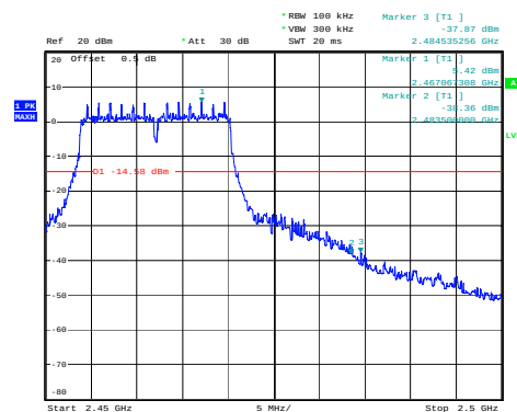
802.11g: Band Edge-High Channel
