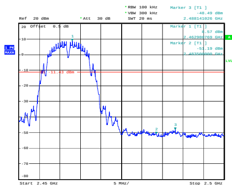
802.11b: Band Edge-High Channel
