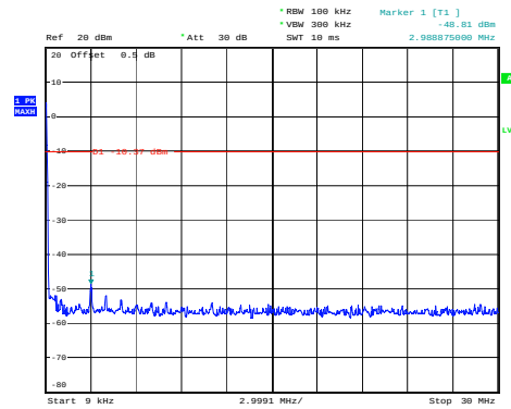
802.11b on channel 01
