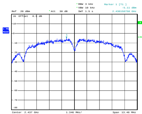
(802.11b) PSD plot on channel 6
