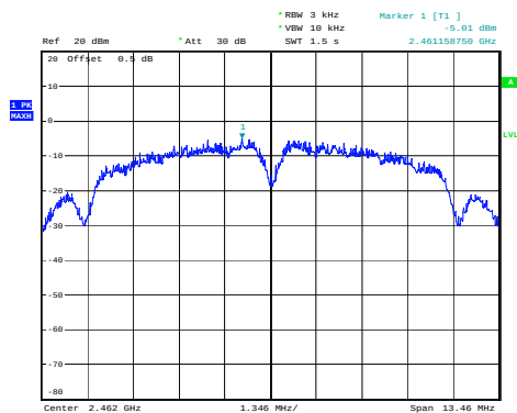
(802.11b) PSD plot on channel 11
