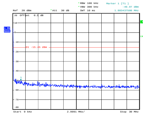
802.11n20 on channel 01
