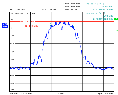
(802.11b) 6dB Bandwidth plot on channel 6
