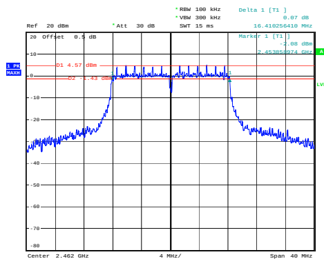
(802.11g) 6dB Bandwidth plot on channel 11
