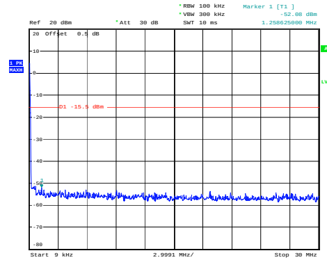
802.11g on channel 11
