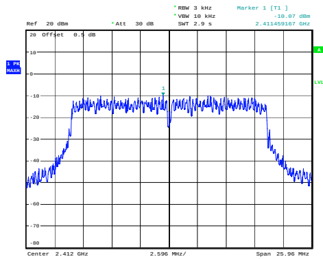
(802.11n20) PSD plot on channel 1
