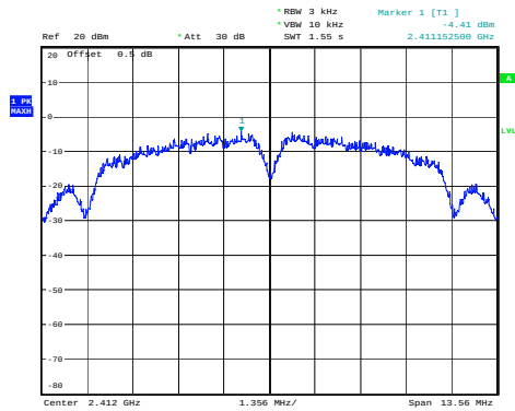
(802.11b) PSD plot on channel 1
