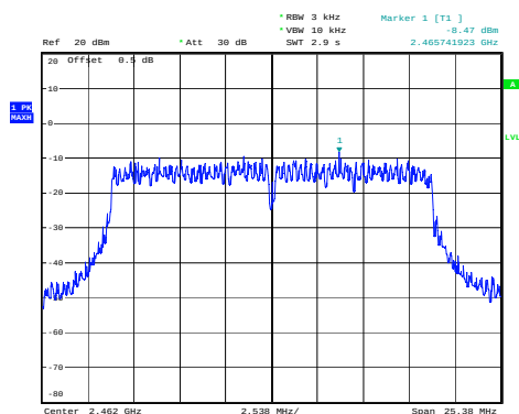
(802.11n20) PSD plot on channel 11
