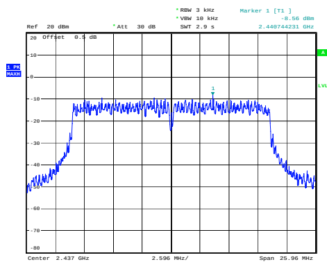
(802.11n20) PSD plot on channel 6
