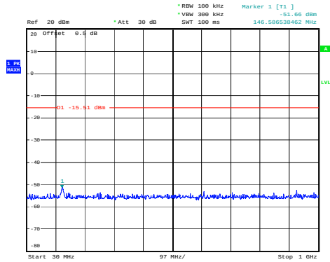
802.11 n20 on channel 11
