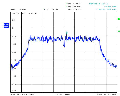
(802.11g) PSD plot on channel 6
