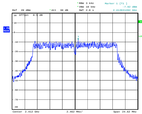
(802.11g) PSD plot on channel 1
