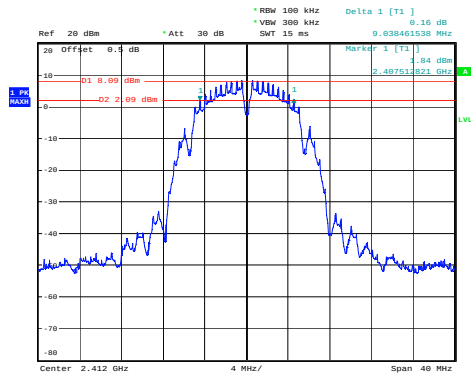
(802.11b) 6dB Bandwidth plot on channel 1
