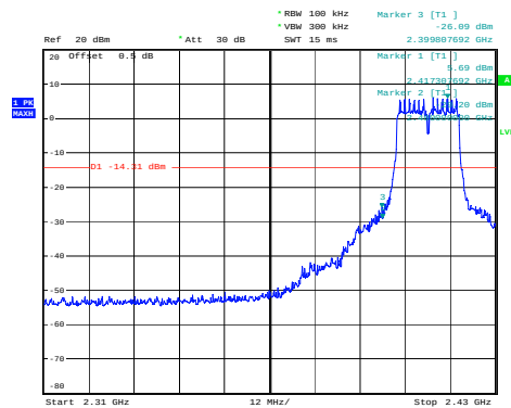
802.11g: Band Edge-Low Channel
