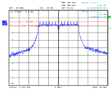
(802.11g) 6dB Bandwidth plot on channel 1
