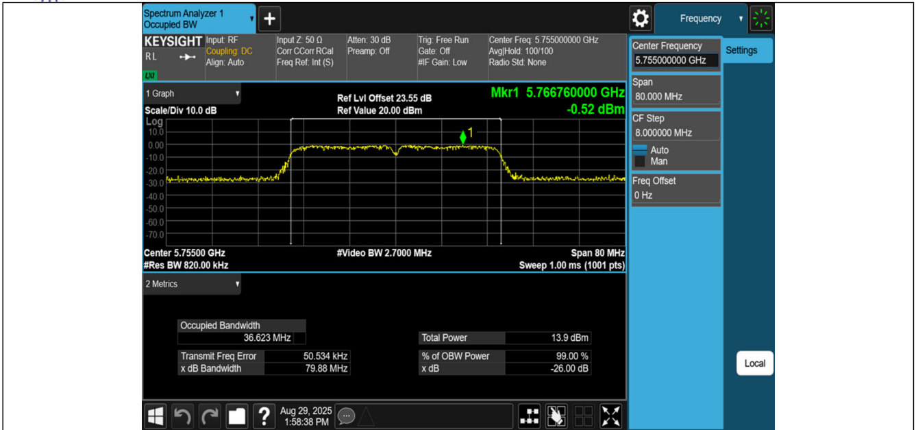
11N40SISO-Ant1-5755
