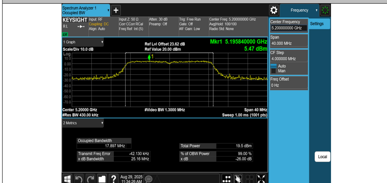
11N20SISO-Ant1-5200
