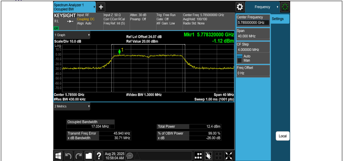
11A-Ant1-5785
