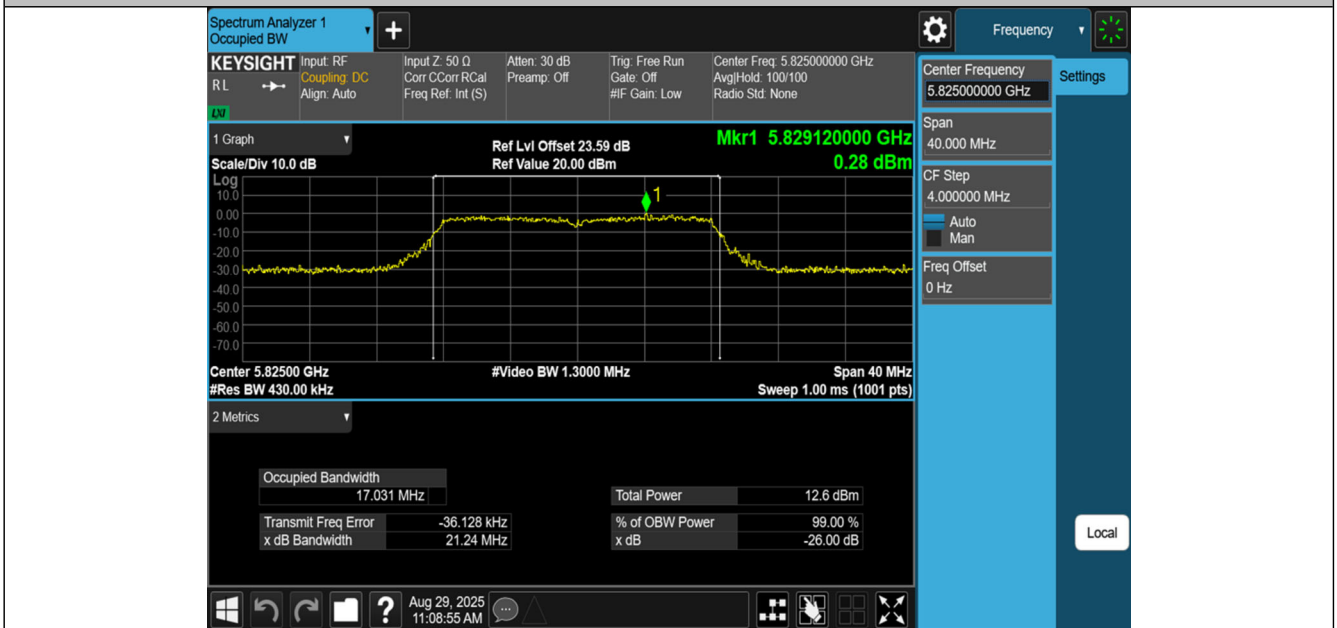
11A-Ant1-5825
