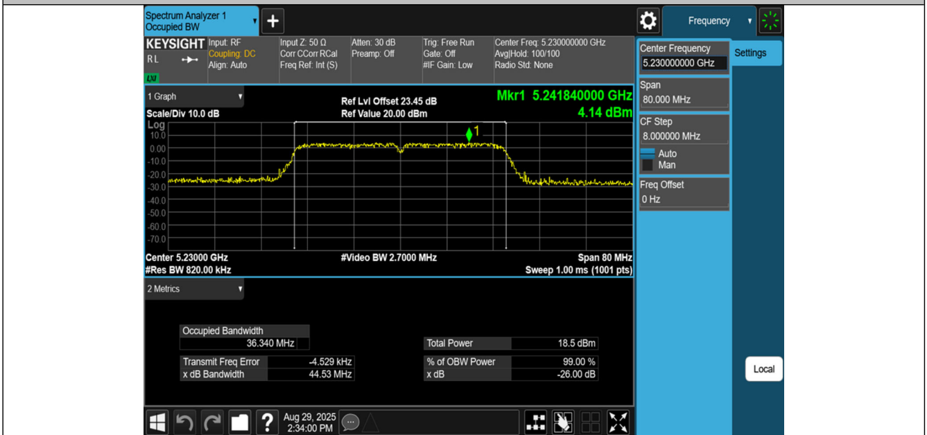
11N40SISO-Ant1-5230
