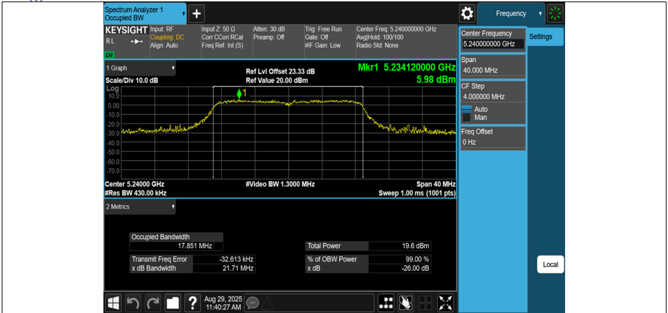
11N20SISO-Ant1-5240
