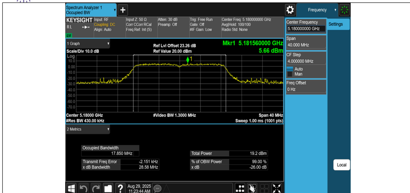
11N20SISO-Ant1-5180
