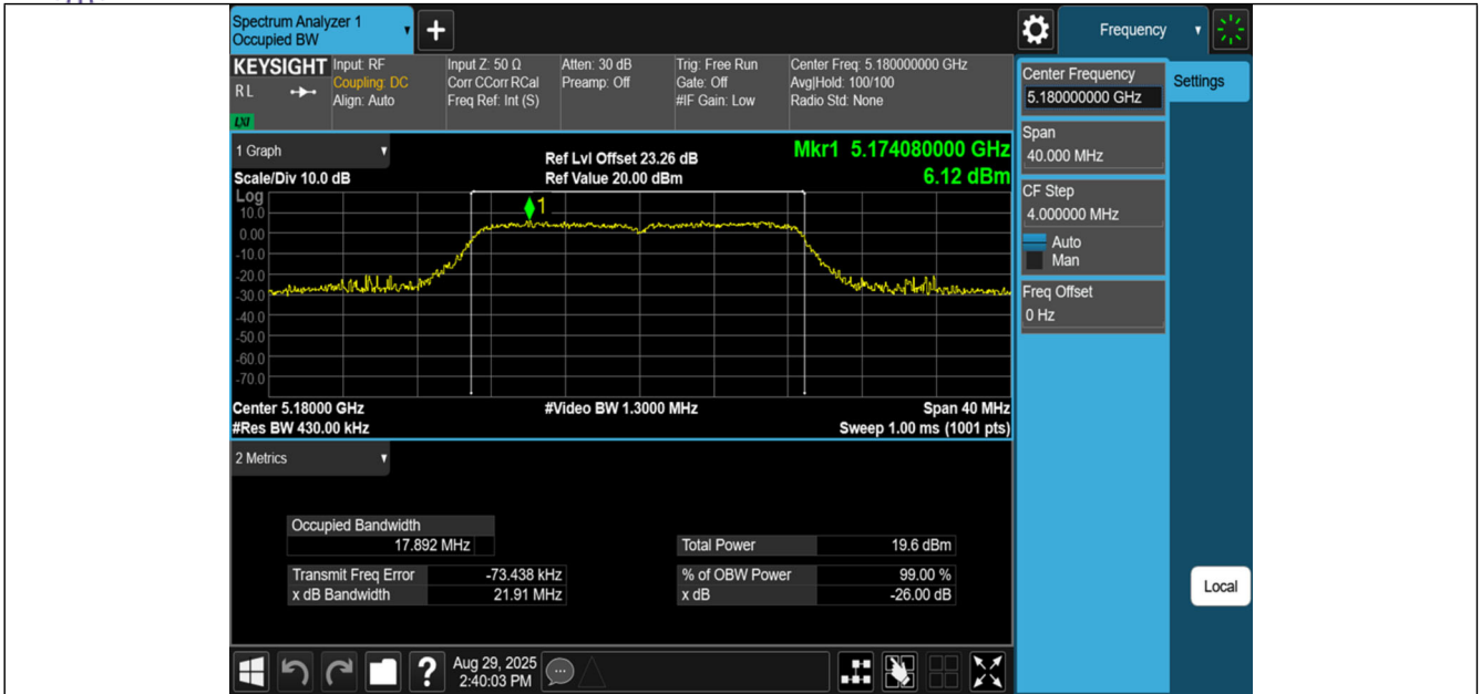
11AC20SISO-Ant1-5180
