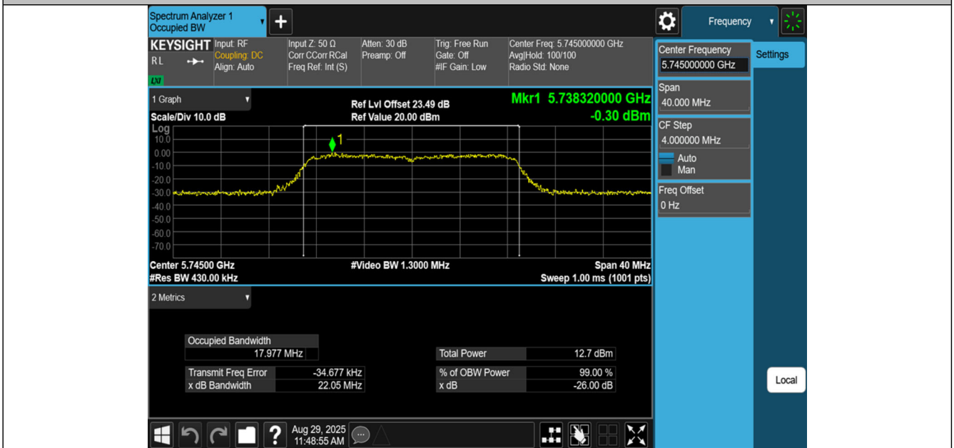
11N20SISO-Ant1-5745
