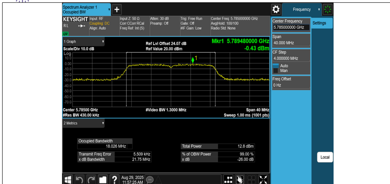
11N20SISO-Ant1-5785
