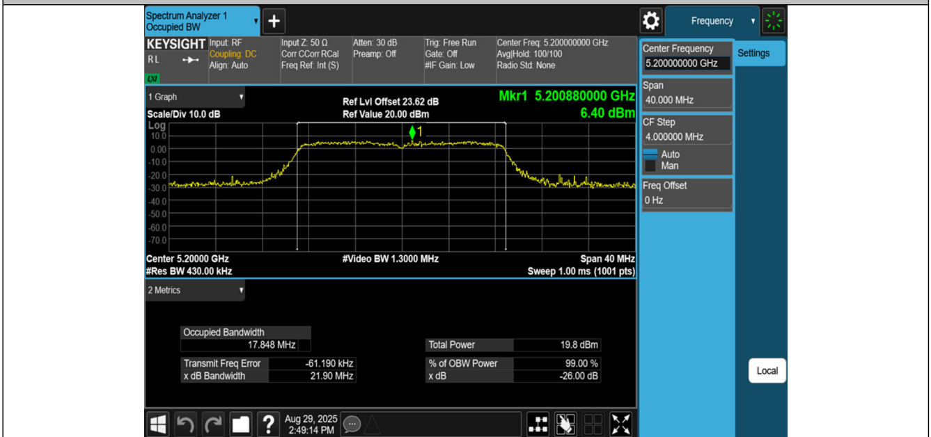
11AC20SISO-Ant1-5200
