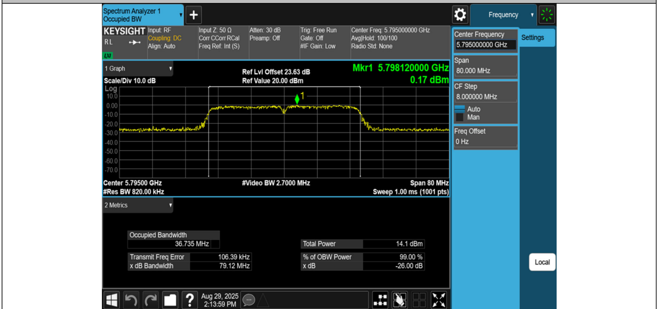
11N40SISO-Ant1-5795
