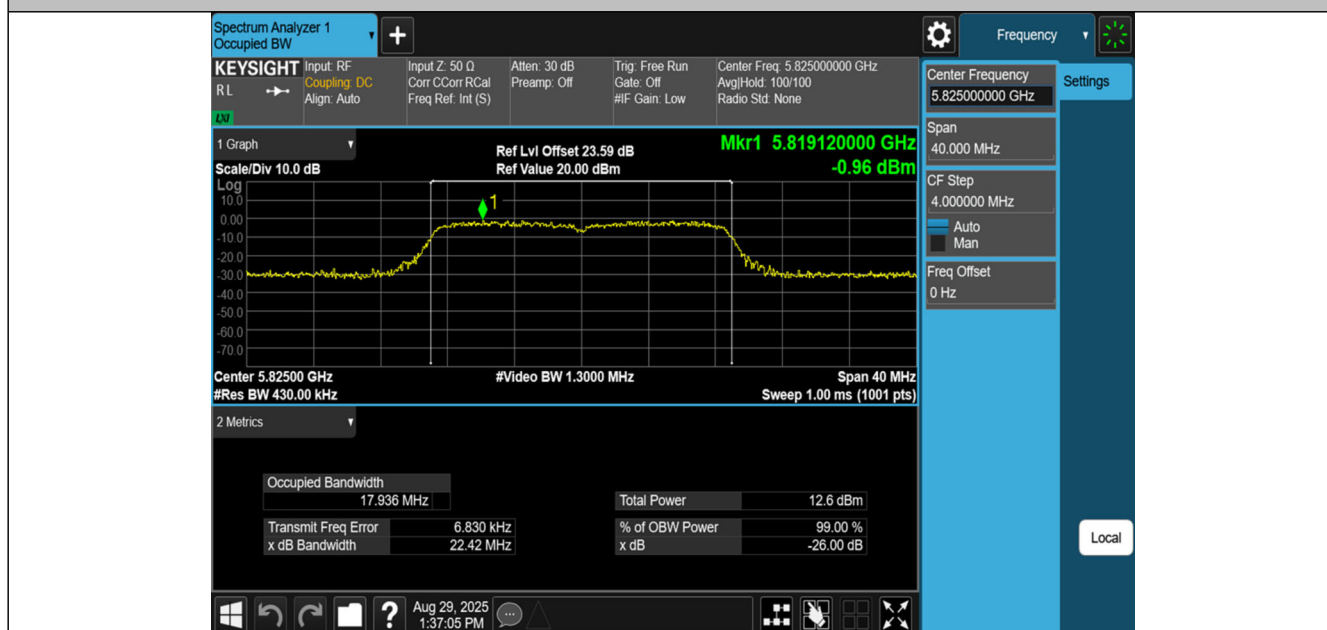
11N20SISO-Ant1-5825
