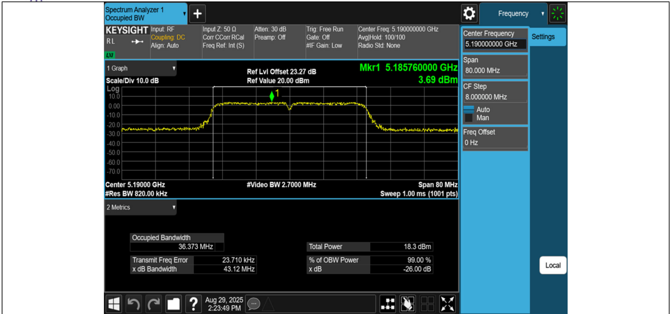
11N40SISO-Ant1-5190
