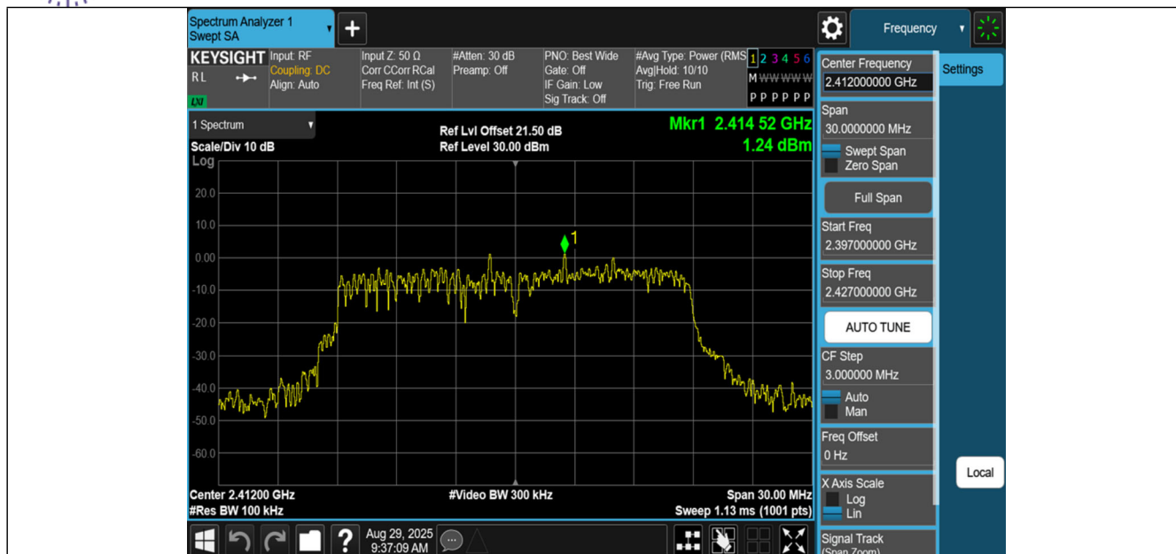
11N20SISO-Ant1-2412-0~Reference-PASS
