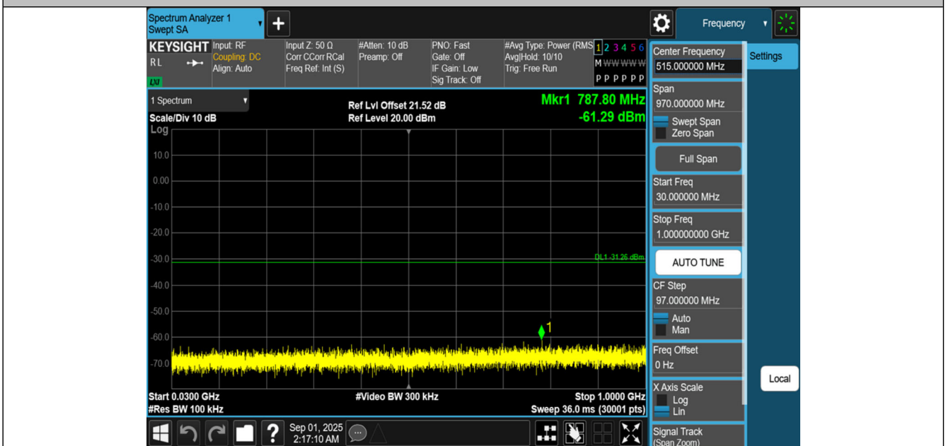
11N40SISO-Ant1-2437-30~1000-PASS
