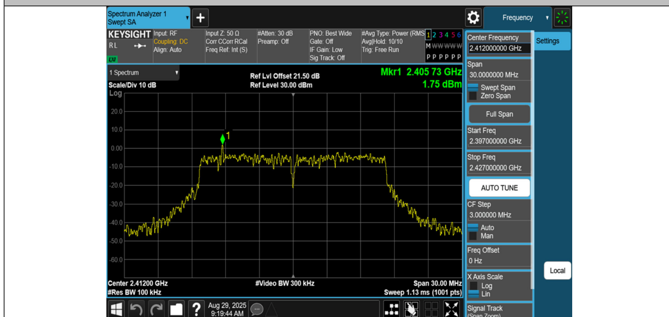
11G-Ant1-2412-0~Reference-PASS
