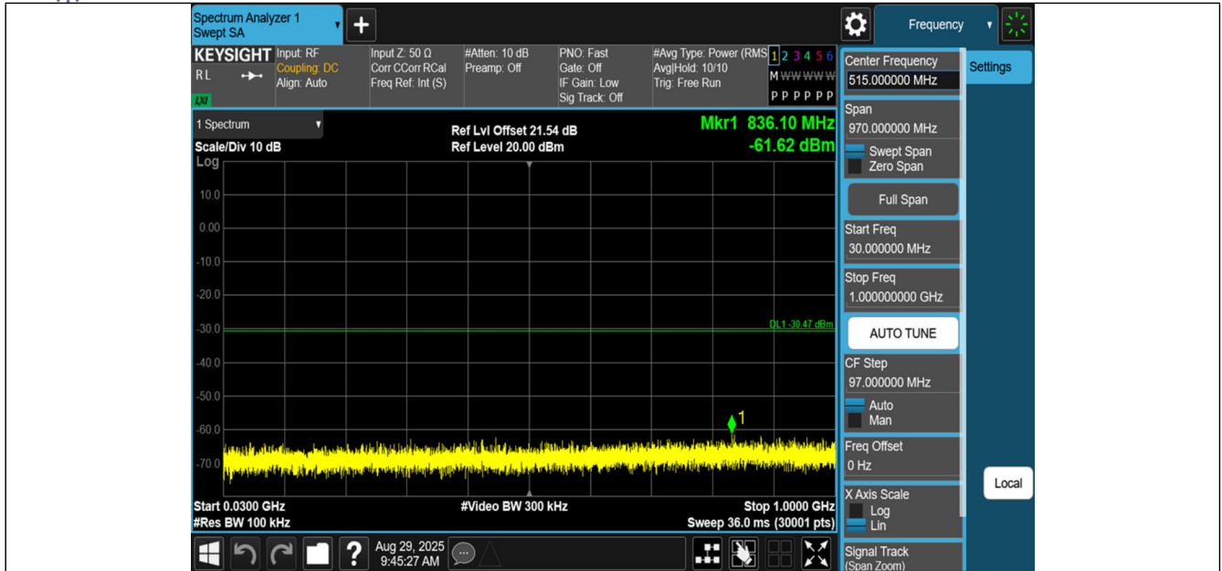
11N40SISO-Ant1-2422-30~1000-PASS
