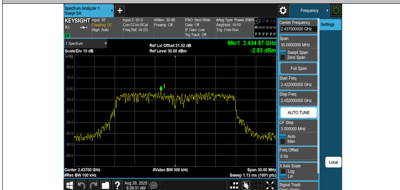
11N20SISO-Ant1-2437-0~Reference-PASS
