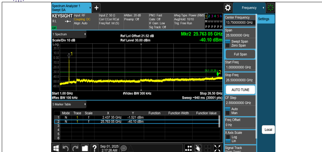
11N40SISO-Ant1-2437-1000~26500-PASS
