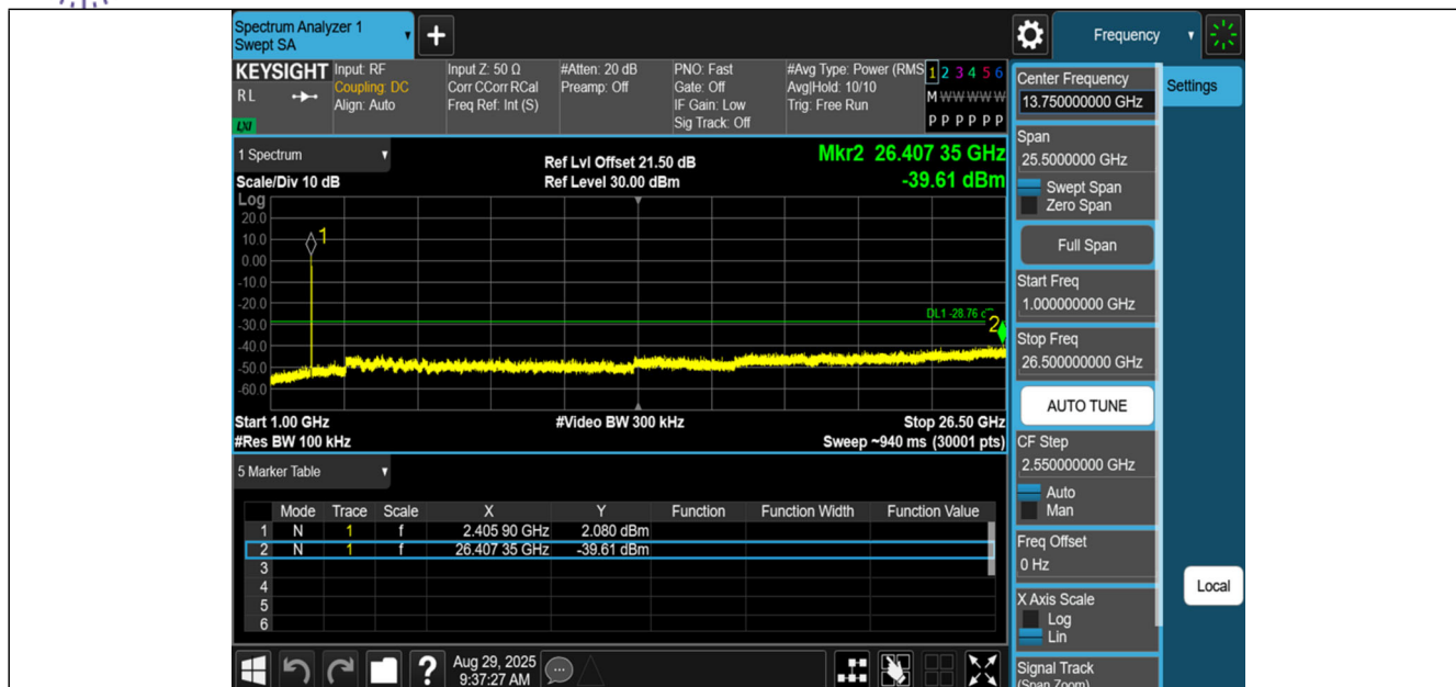
11N20SISO-Ant1-2412-1000~26500-PASS
