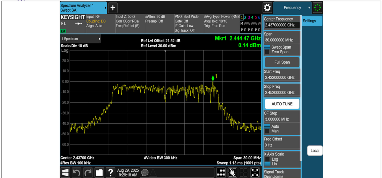
11G-Ant1-2437-0~Reference-PASS
