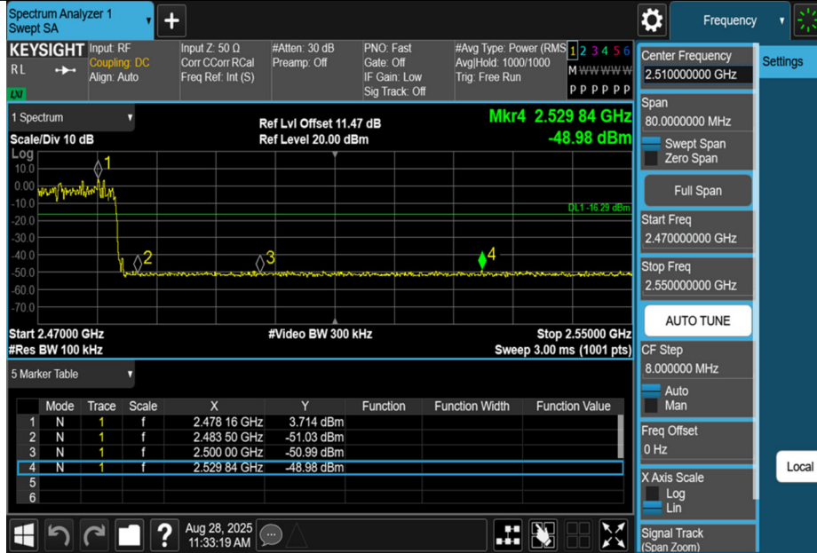
3DH5-Ant1-Hop_2480-PASS
