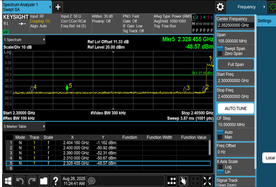
2DH5-Ant1-Hop_2402-PASS
