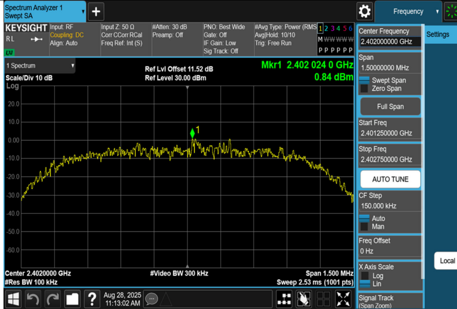
3DH5-Ant1-2402-0~Reference-PASS
