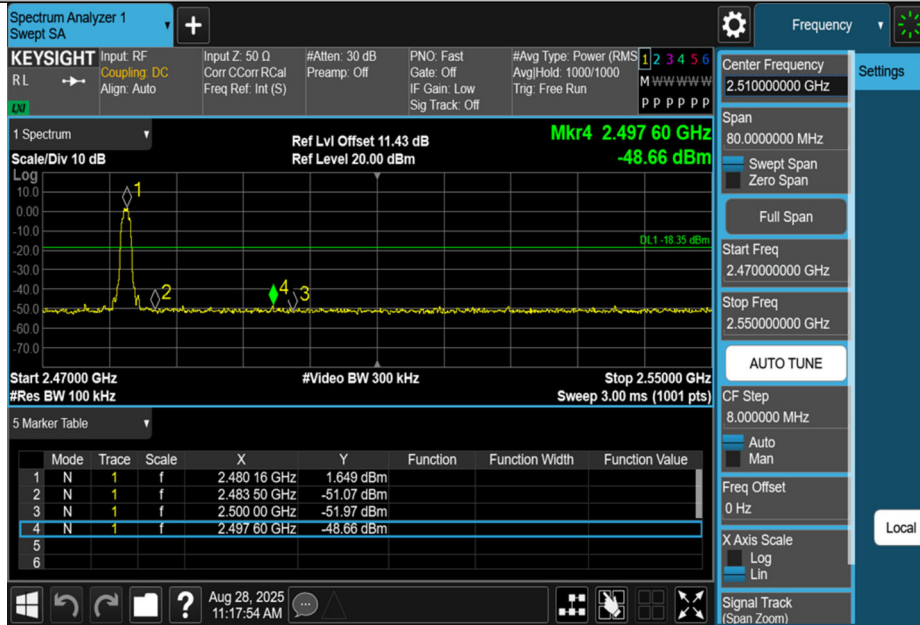
3DH5-Ant1-2480-PASS
