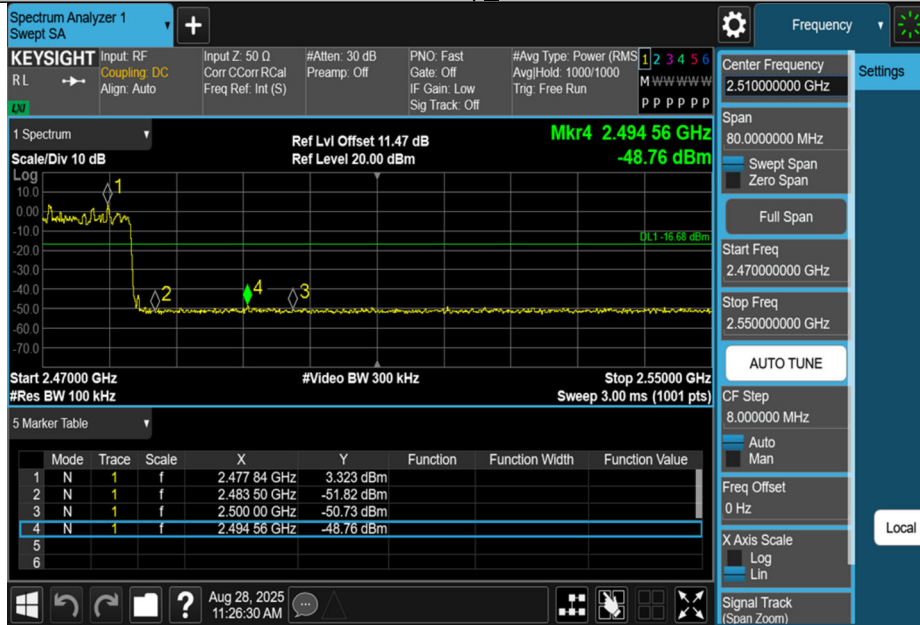
2DH5-Ant1-Hop_2480-PASS
