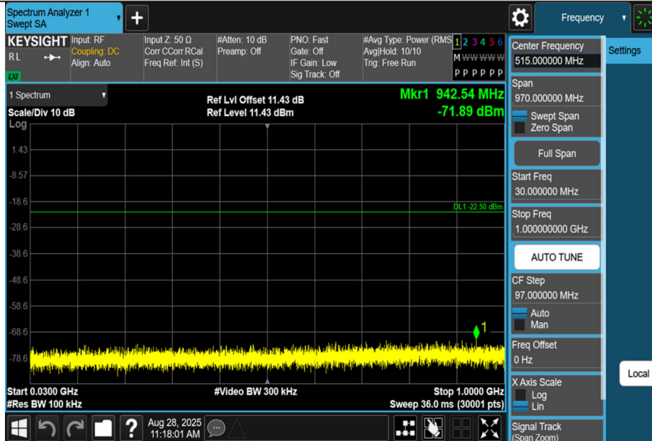
3DH5-Ant1-2480-30~1000-PASS
