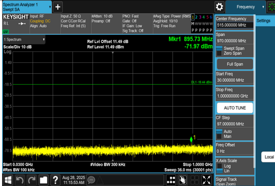
3DH5-Ant1-2441-30~1000-PASS
