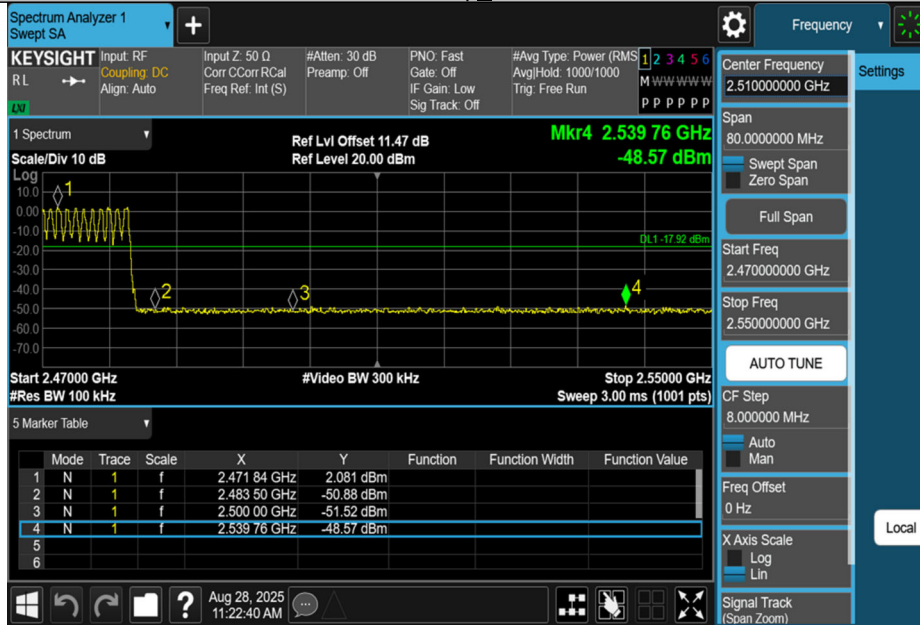
DH5-Ant1-Hop_2480-PASS
