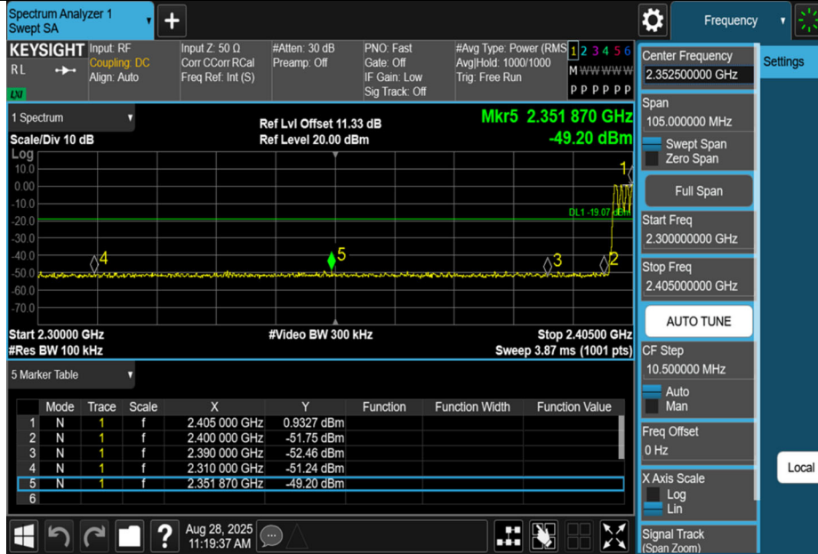
DH5-Ant1-Hop_2402-PASS
