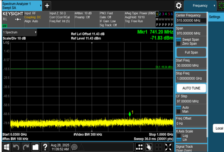
2DH5-Ant1-2480-30~1000-PASS
