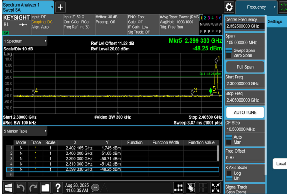
2DH5-Ant1-2402-PASS
