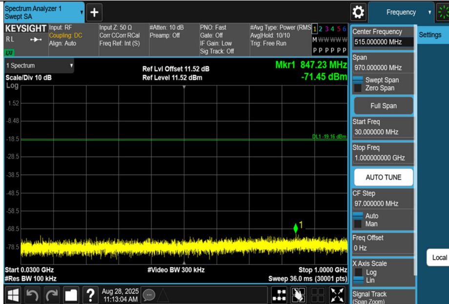
3DH5-Ant1-2402-30~1000-PASS
