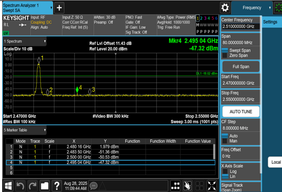
2DH5-Ant1-2480-PASS
