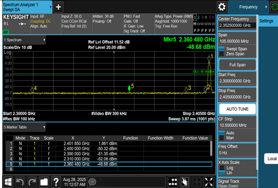
3DH5-Ant1-2402-PASS
