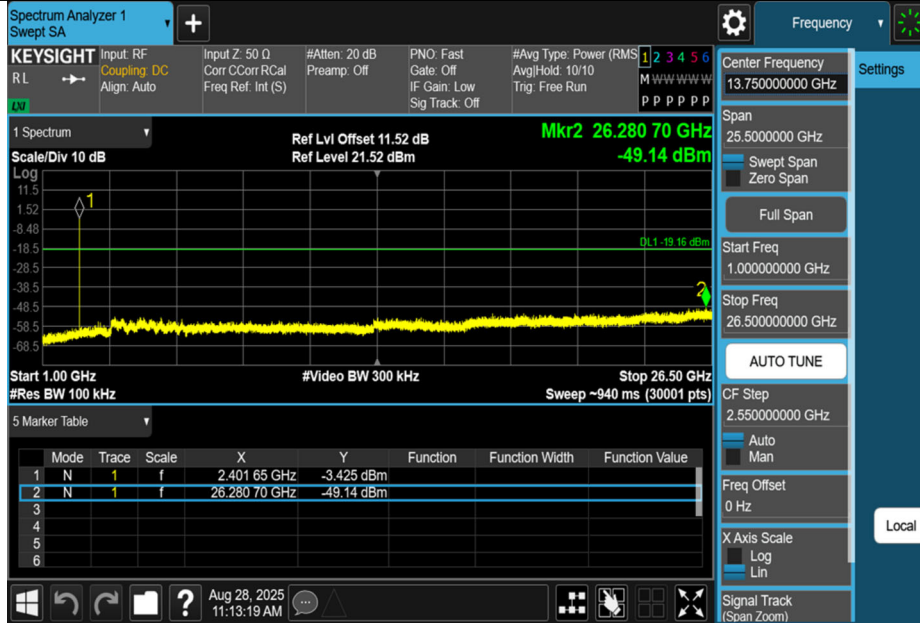
3DH5-Ant1-2402-1000~26500-PASS
