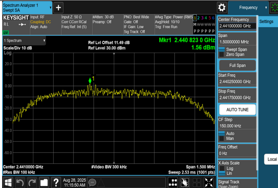
3DH5-Ant1-2441-0~Reference-PASS
