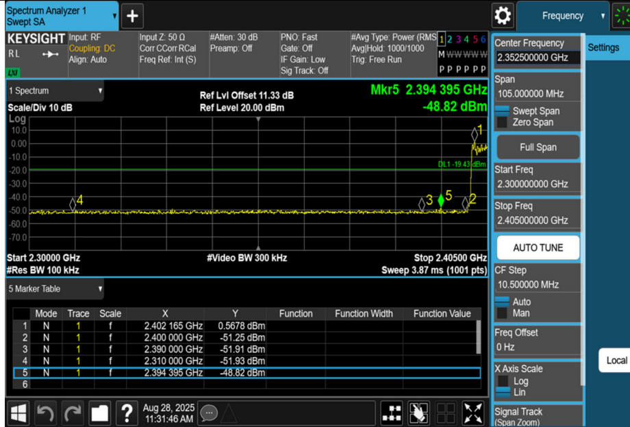
3DH5-Ant1-Hop_2402-PASS
