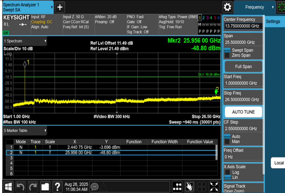
2DH5-Ant1-2441-1000~26500-PASS
