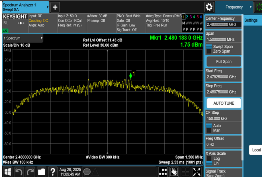
2DH5-Ant1-2480-0~Reference-PASS
