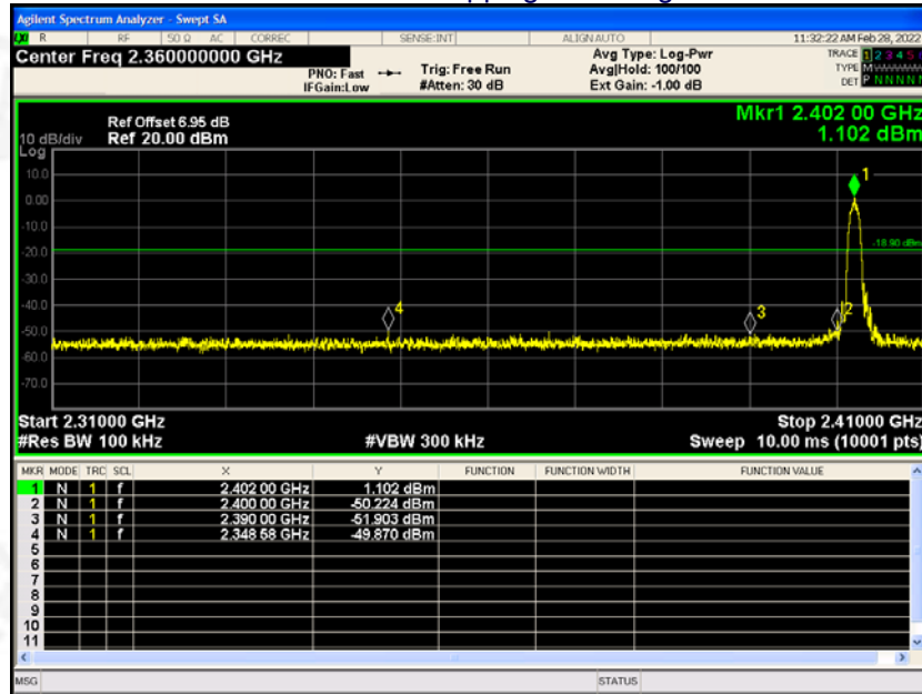
\pi/4 DQPSK No-hopping Band edge-left side
