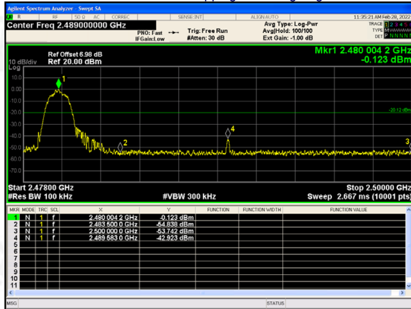
\pi/4 DQPSK No-hopping Band edge-right side
