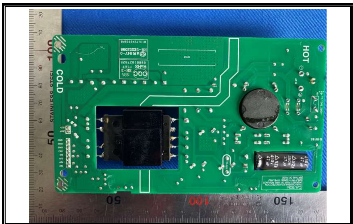
Internal view - Power board Bottom
