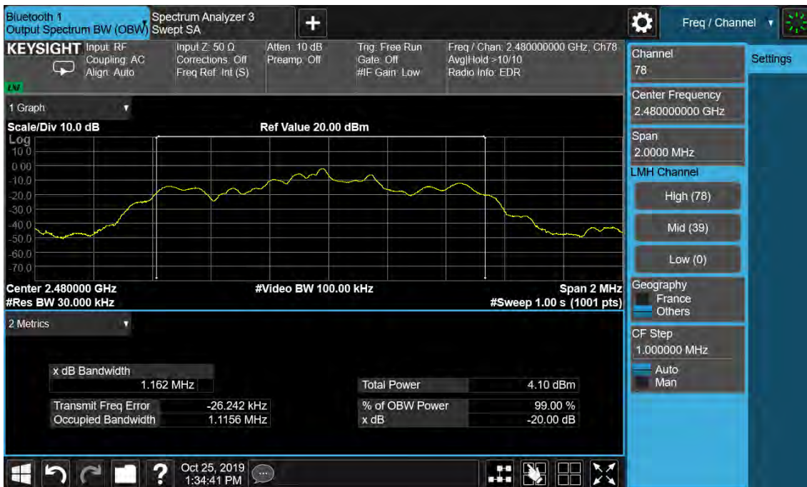
Figure 15: 20dB Bandwidth and 99% Bandwidth, 2480MHz, 8-DPSK
