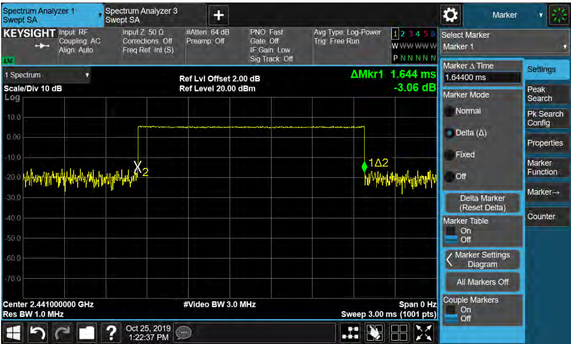
Figure 29: Time of Occupancy, 2441MHz, GFSK DH3
