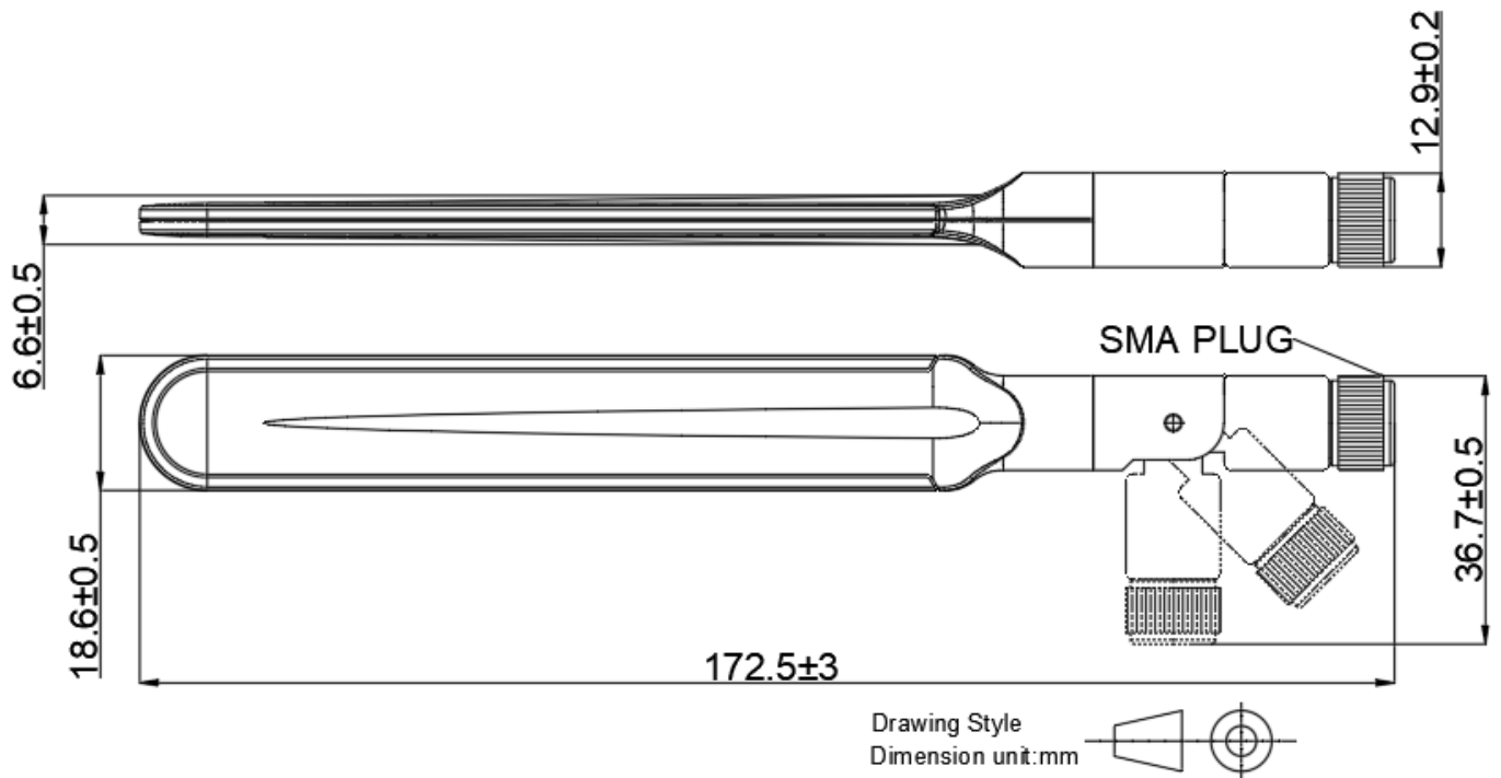
Figure 6: Model DPD2450APB Dimensions
