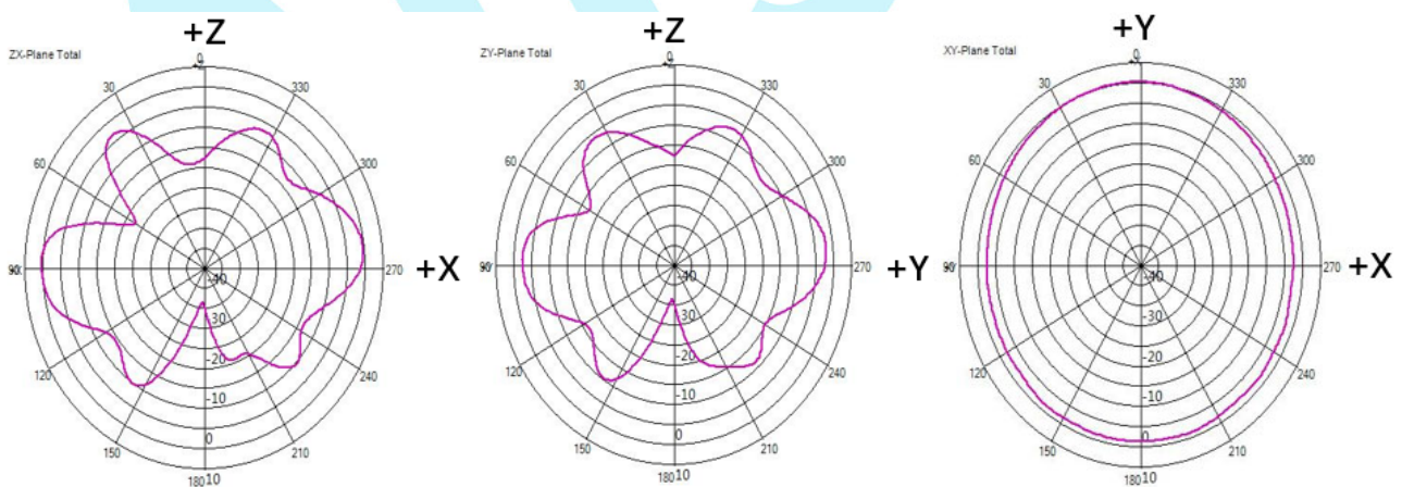
Figure 5: Model DPD2450APB Radiation Patterns at 5.55GHz
