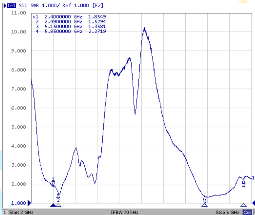
Figure 2: Model DPD2450APB VSWR
