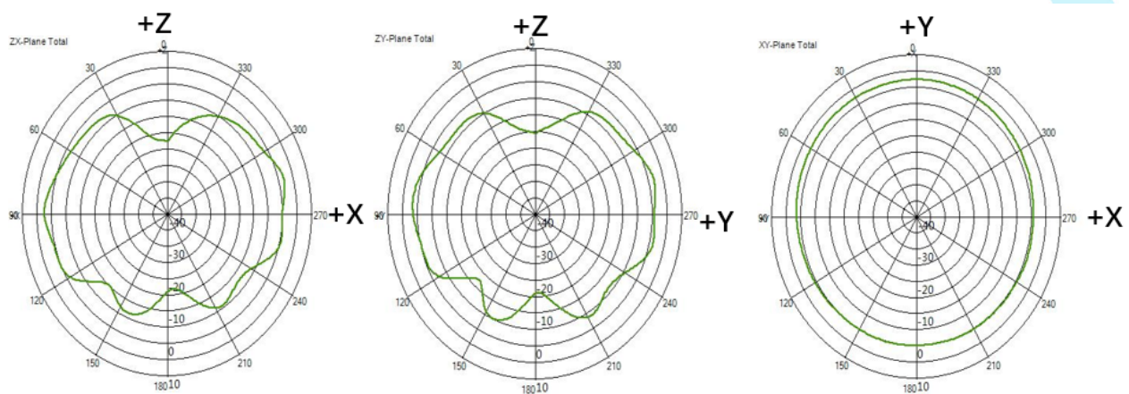
Figure 4: Model DPD2450APB Radiation Patterns at 2.44GHz
