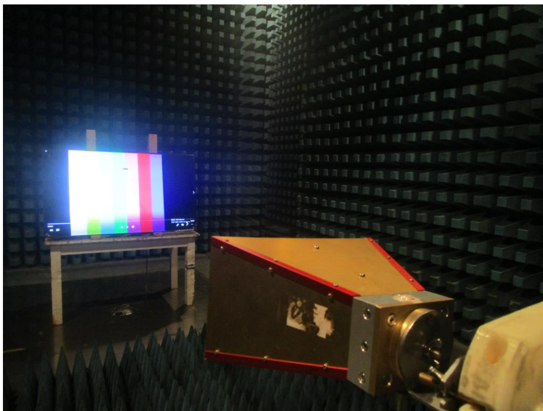
Note: the EUT's antenna 1.5m from the floor
