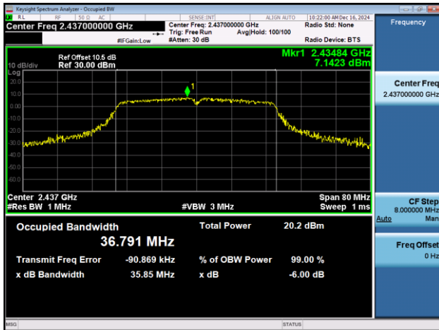
11AX40SISO-Ant1-2437
