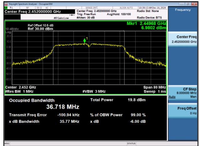
11AX40SISO-Ant1-2452
