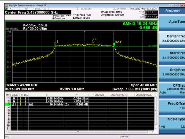
11G-Ant1-2437-PASS
