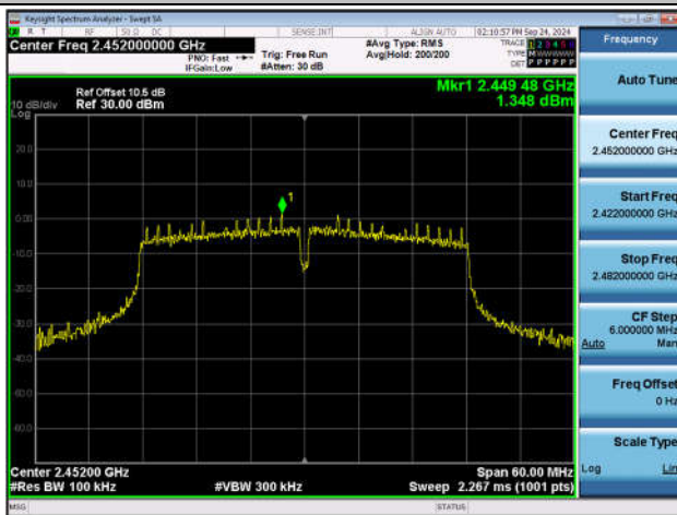
11AX40SISO-Ant1-2452-0~Reference-PASS
