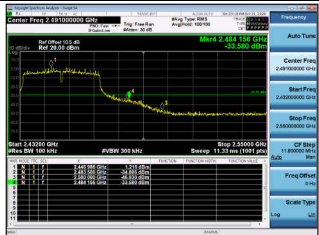
11AX20SISO-Ant1-2462-PASS
