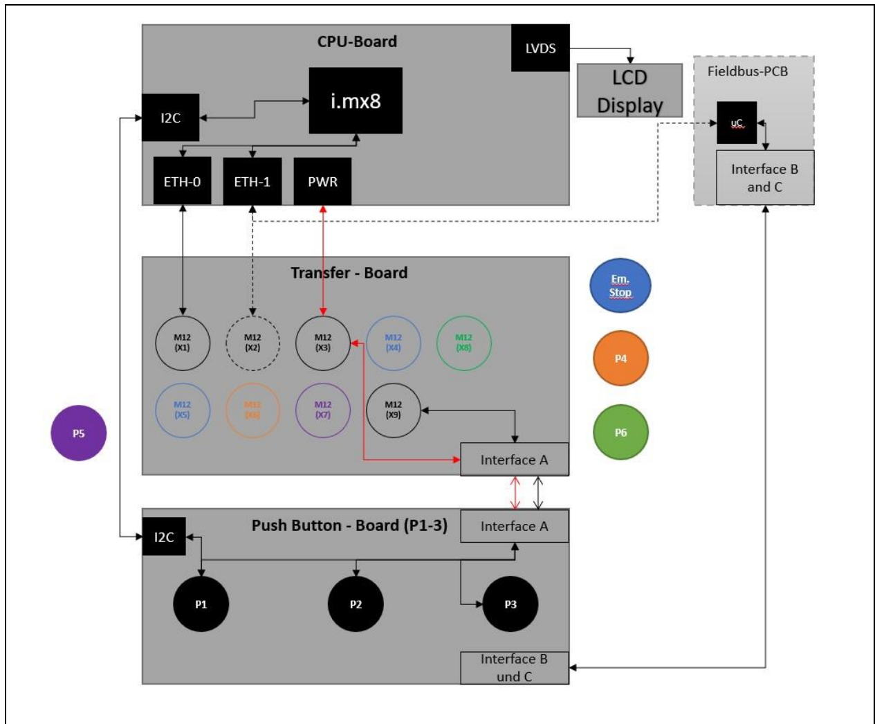
Figure 4-3: Block diagram of function
