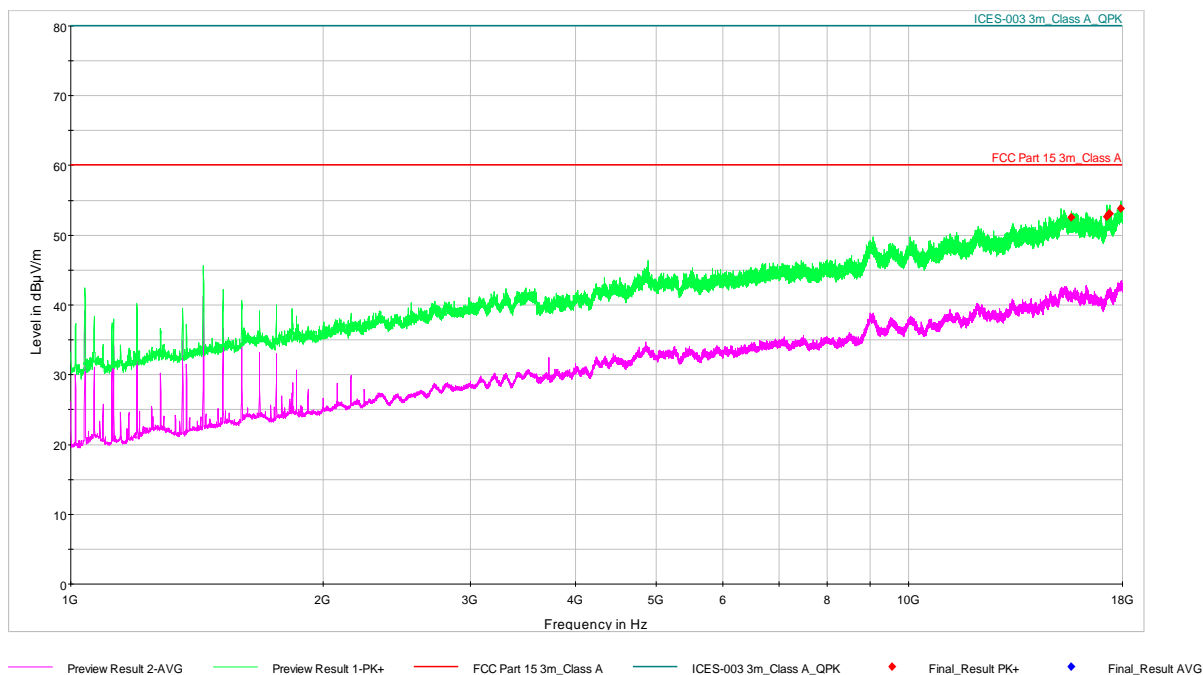
Figure 6-7: Graphical presentation Radiated disturbances 1 GHz to 18 GHz
