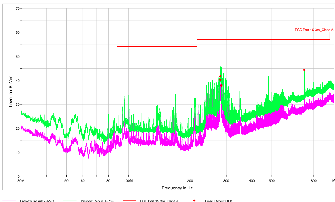
Figure 6-5: Graphical presentation Radiated disturbances 30 MHz to 1000 MHz
