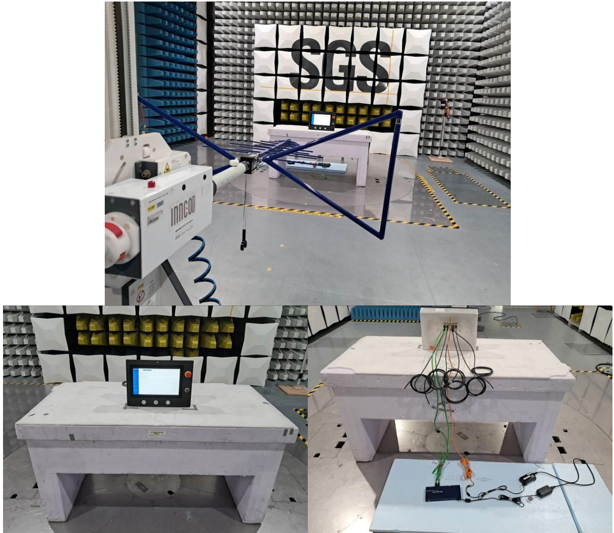
Figure 6-4: test setup for Radiated disturbances 30 MHz to 1000 MHz
