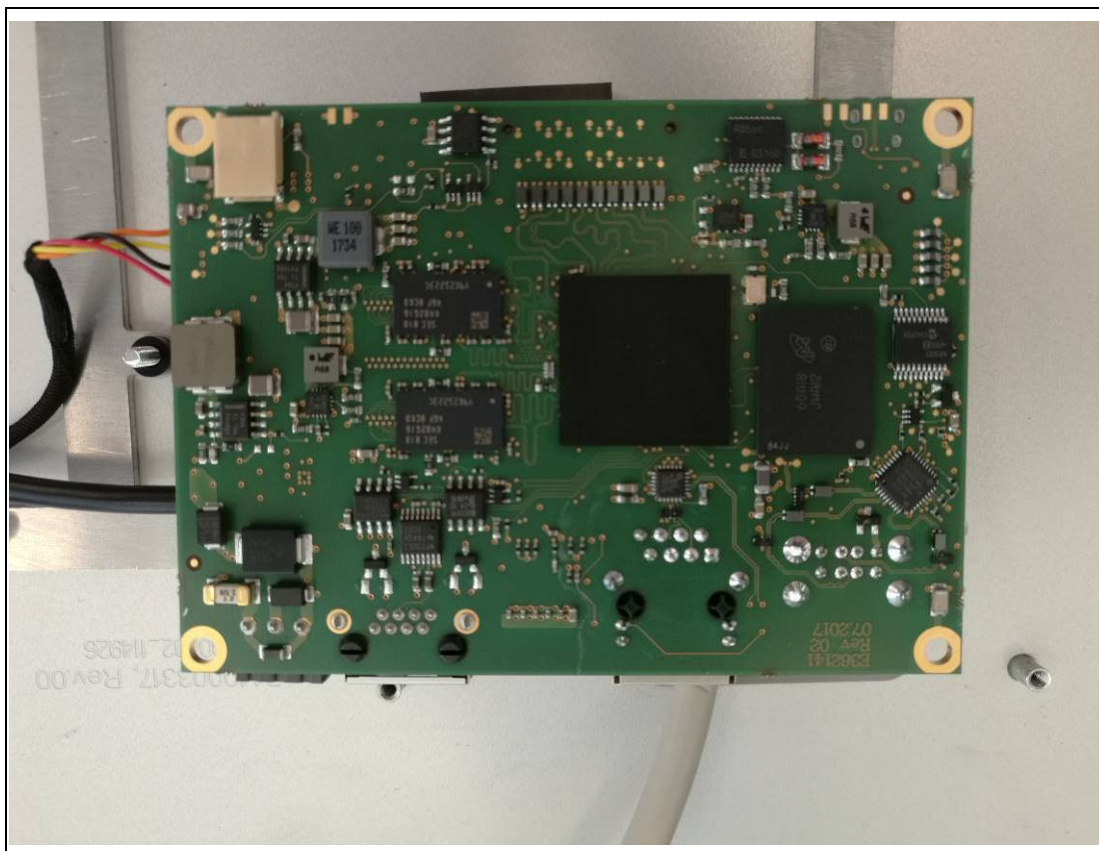
Figure 3: Rear view of Main board of Touch-it CE VESA glass 15,6
