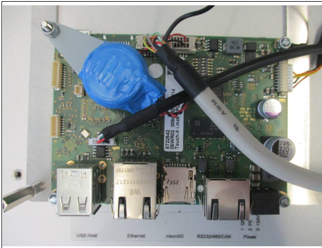
Figure 2: Front view of Main board of Touch-it CE VESA glass 15,6
