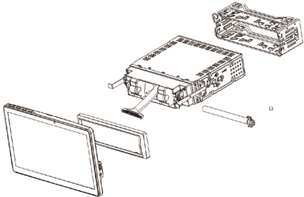
TYPICAL FRONT-LOAD DIN MOUNTING METHOD
