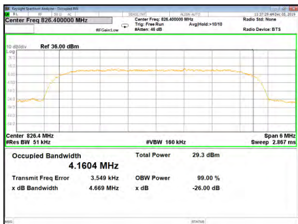
B5_WCDMA_Lower_26BW and 99%
