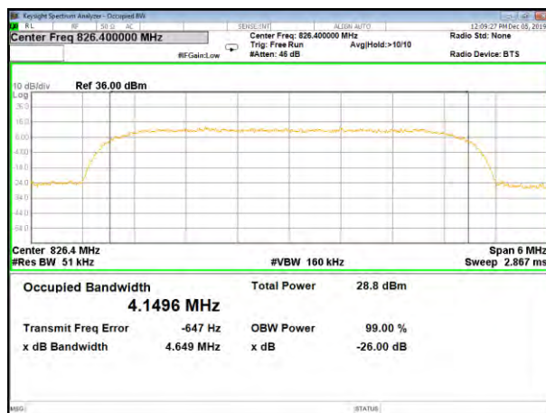
B5_HSDPA_Lower_26BW and 99%
