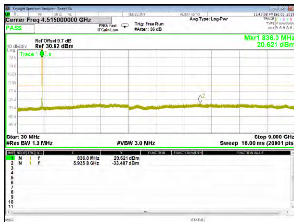
B5_HSUPA_Middle_Conducted Spurious
