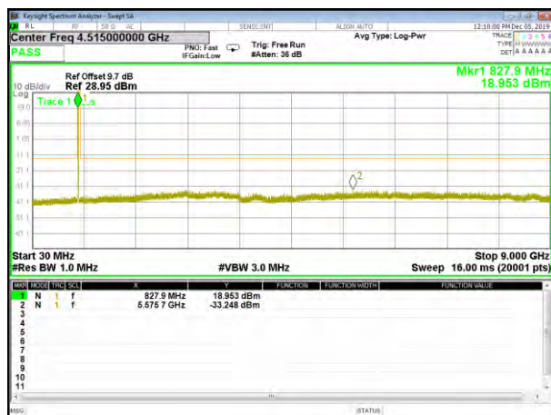
B5_HSDPA_Lower_Conducted Spurious
