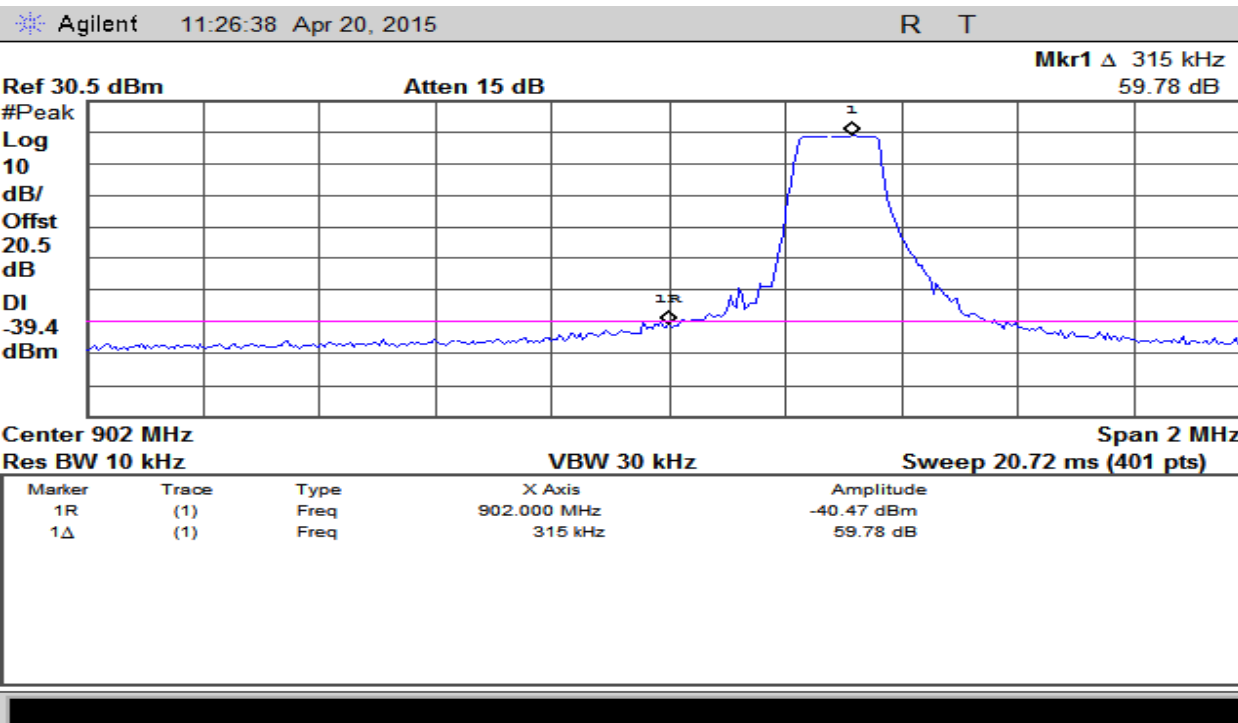
Plot 24 - Band Edge – Low Channel – Hybrid Mode
