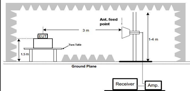
Above 1GHz
