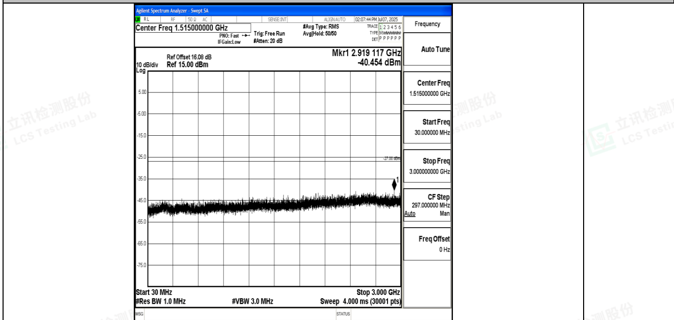
11AX20SISO-Ant1-6435-30~3000-PASS
