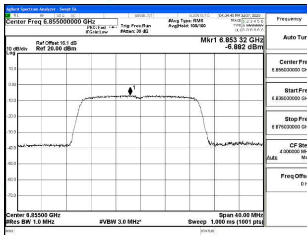
11AX20SISO-Ant1-6855-PASS
