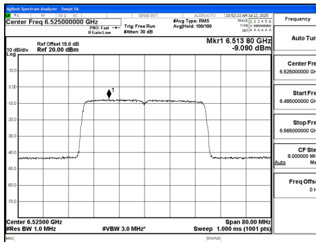
11AX40SISO-Ant1-6525-PASS
