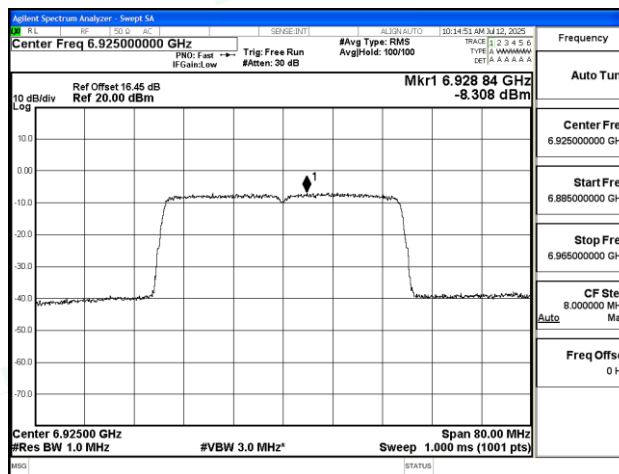
11AX40SISO-Ant2-6925-PASS
