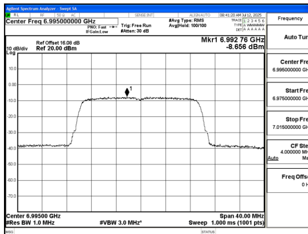
11AX20SISO-Ant1-6995-PASS
