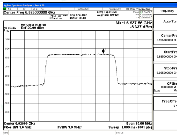
11AX40SISO-Ant1-6925-PASS
