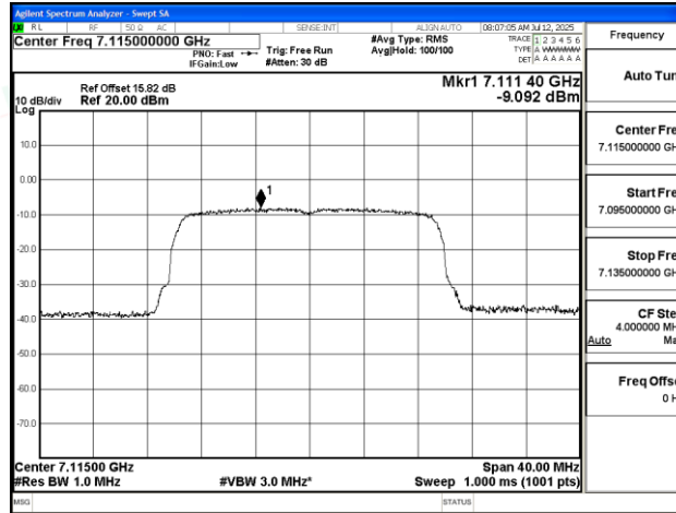
11AX20SISO-Ant1-7115-PASS
