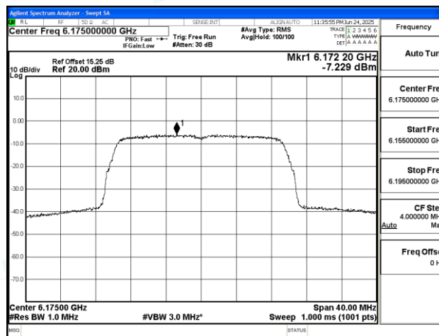
11AX20SISO-Ant2-6175-PASS
