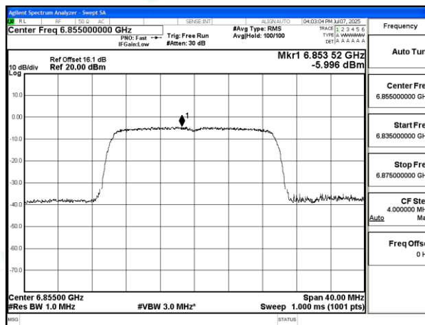
11AX20SISO-Ant2-6855-PASS
