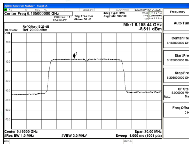
11AX40SISO-Ant1-6165-PASS
