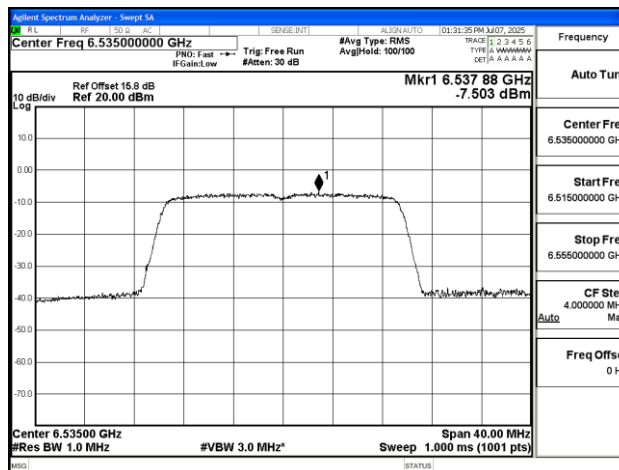
11AX20SISO-Ant1-6535-PASS
