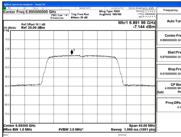
11AX20SISO-Ant1-6895-PASS
