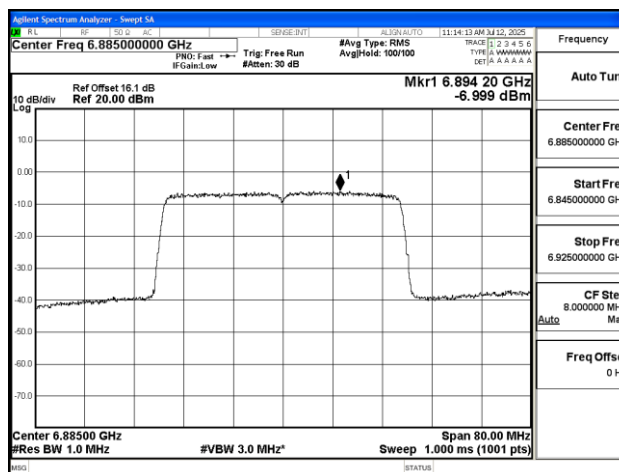
11AX40SISO-Ant2-6885-PASS
