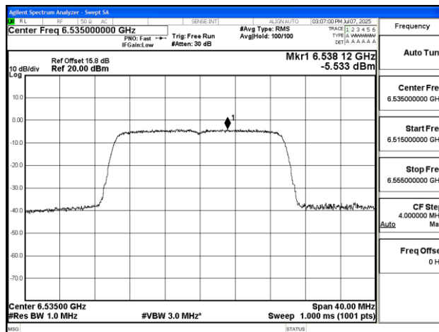
11AX20SISO-Ant2-6535-PASS
