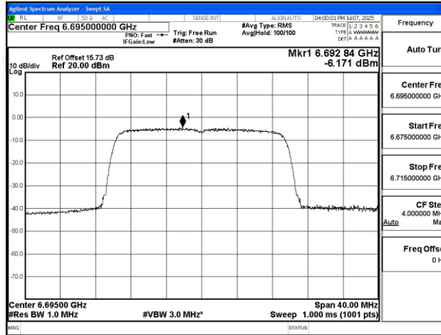
11AX20SISO-Ant2-6695-PASS
