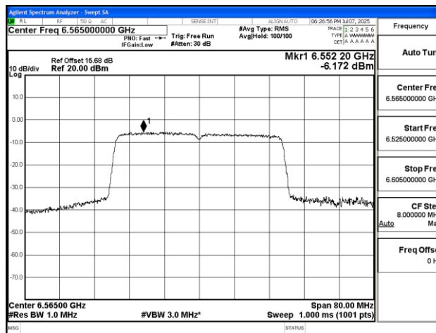
11AX40SISO-Ant2-6565-PASS
