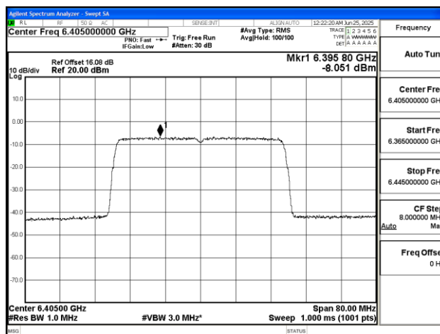
11AX40SISO-Ant2-6405-PASS
