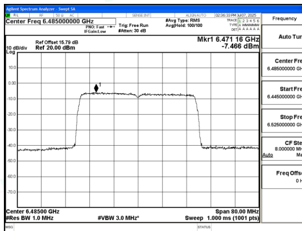
11AX40SISO-Ant1-6485-PASS
