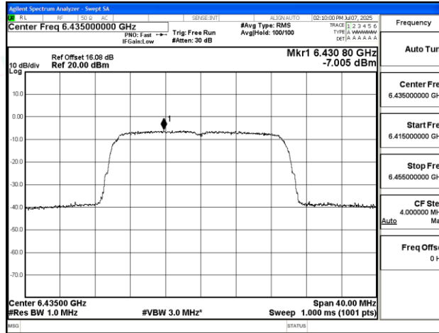
11AX20SISO-Ant2-6435-PASS
