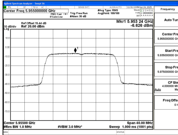
11AX20SISO-Ant2-5955-PASS
