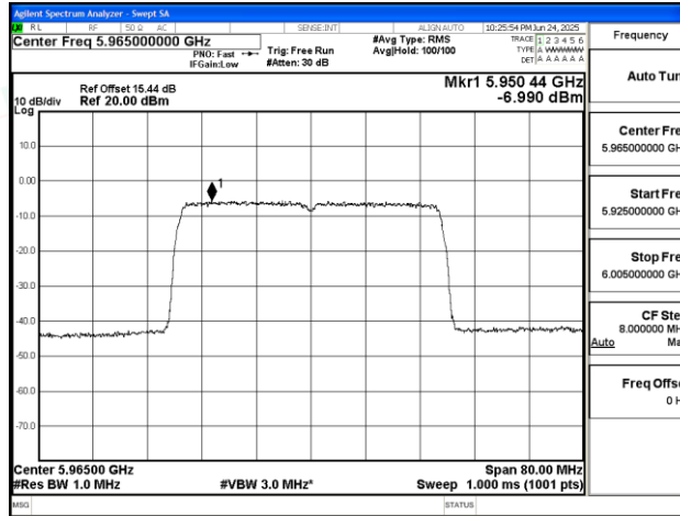
11AX40SISO-Ant1-5965-PASS
