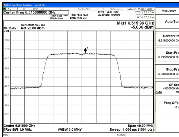
11AX20SISO-Ant2-6515-PASS
