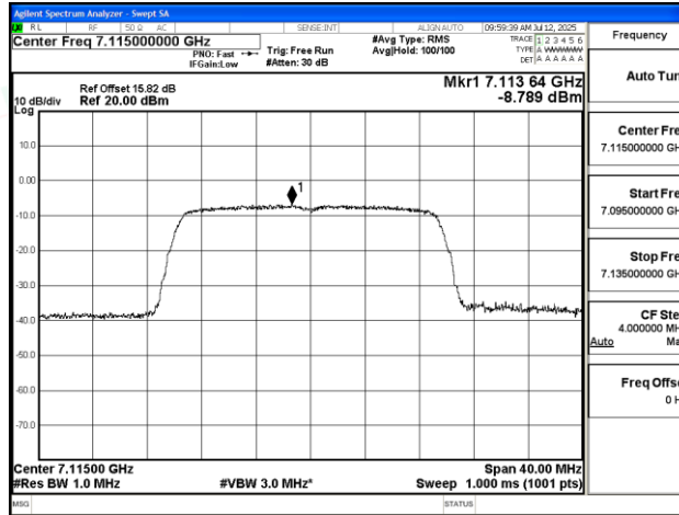
11AX20SISO-Ant2-7115-PASS
