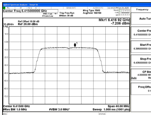
11AX20SISO-Ant2-6415-PASS
