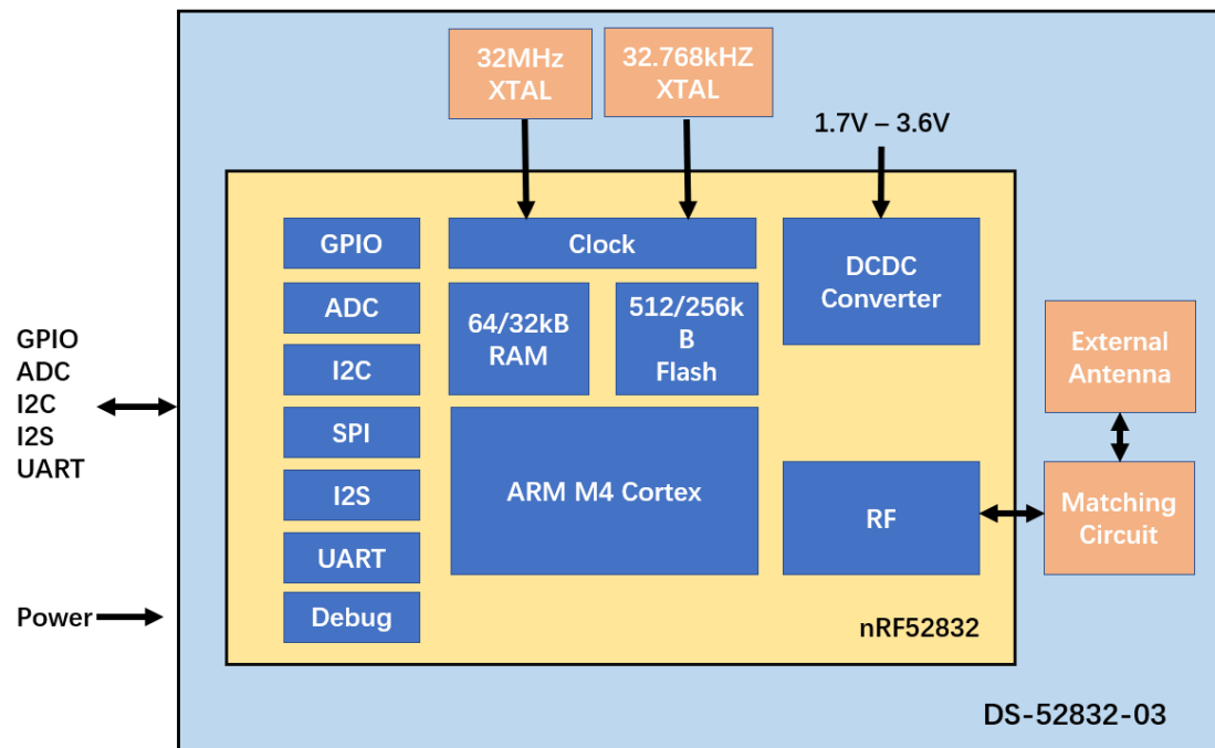
<Figure 2.Simplified block diagram of DS-52832-03>
