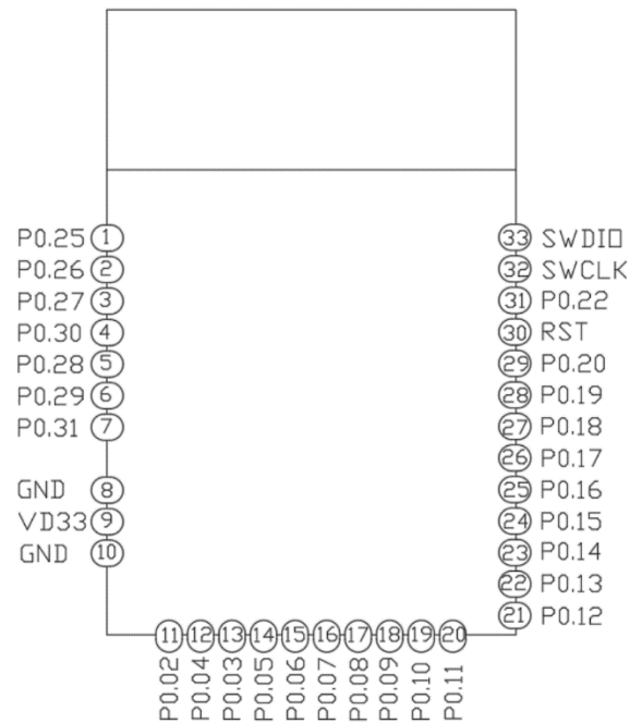
<Figure 4. PIN descriptions>
