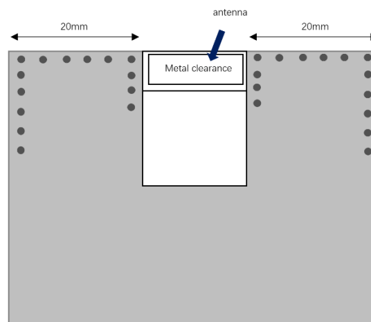
<Figure 7. PCBA design drawing>
