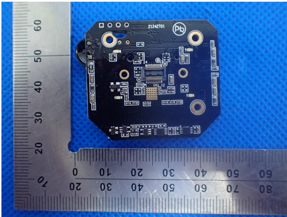
INTERNAL VIEW OF EUT(FIGURE 25)
