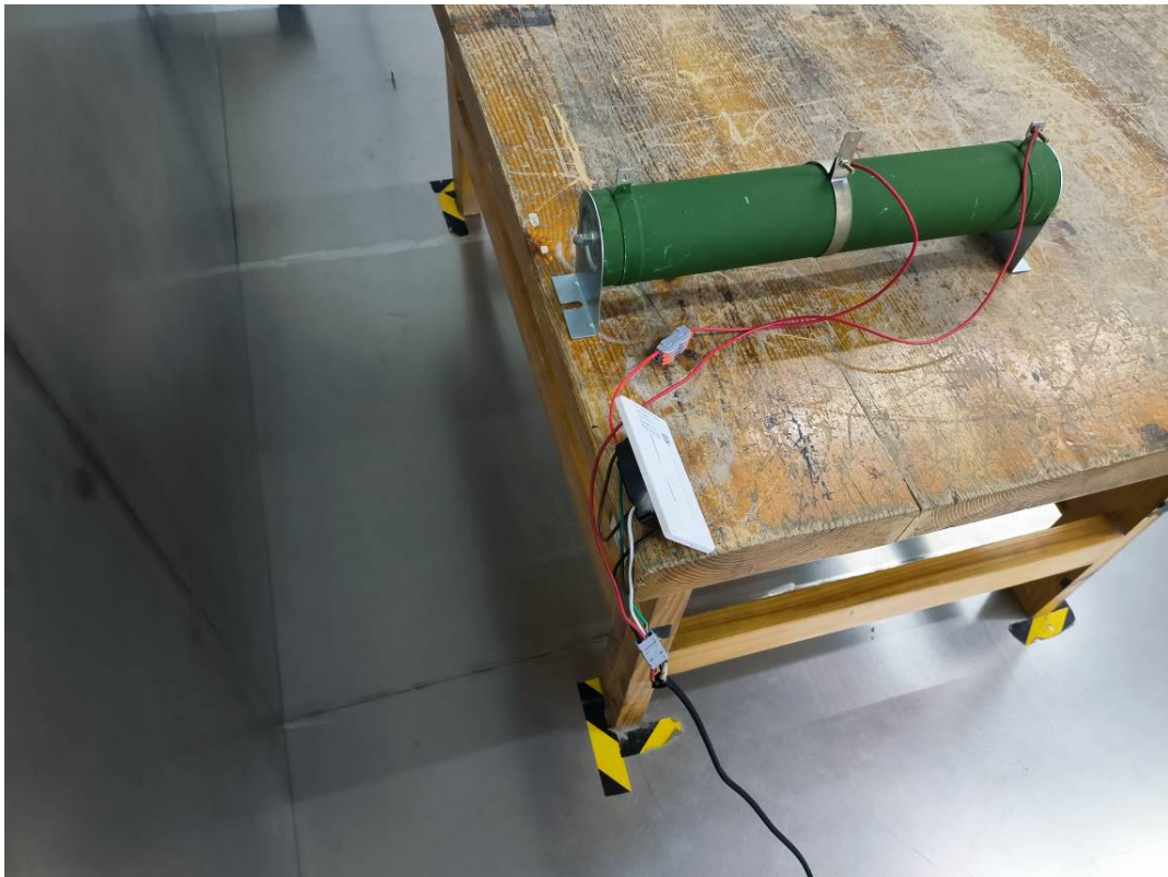
Conducted Emissions Side View- SNA042CLR2-W-1X600-P
