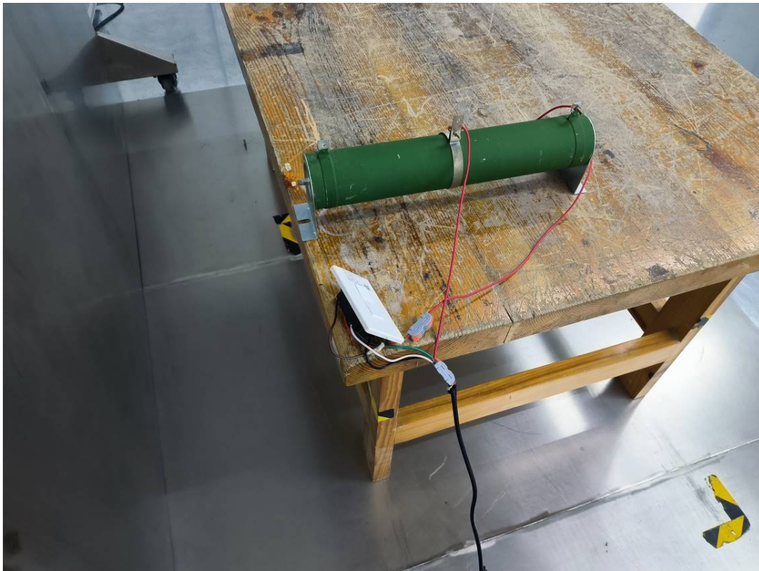
Conducted Emissions Side View-SNA042CLR2-W-1X1200-P
