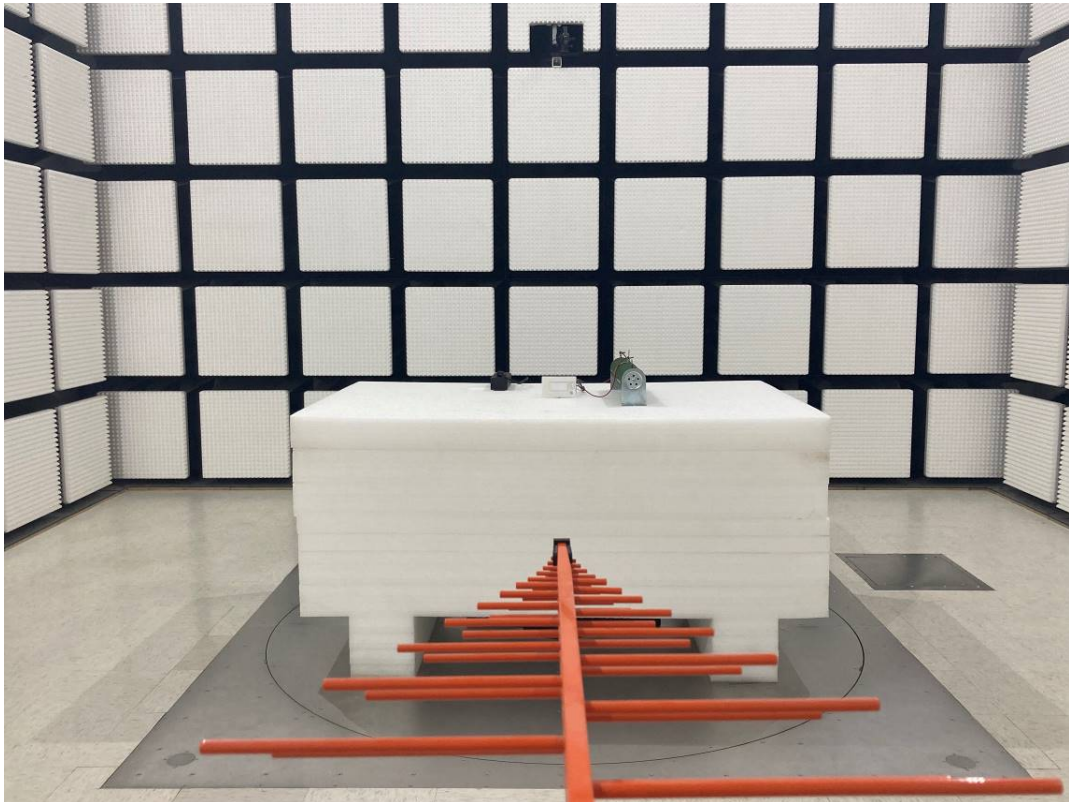
Radiated Emission Below 1GHz View- SNA042CLR2-W-1X600-P
