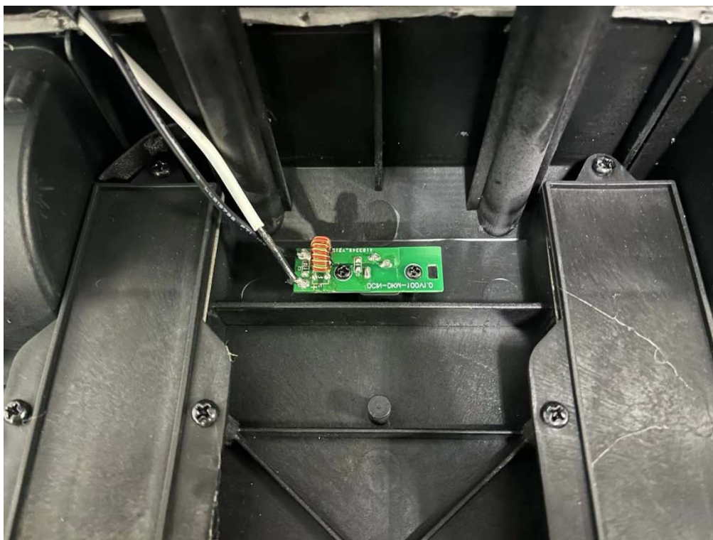
Internal photos M/N: DKM-100
