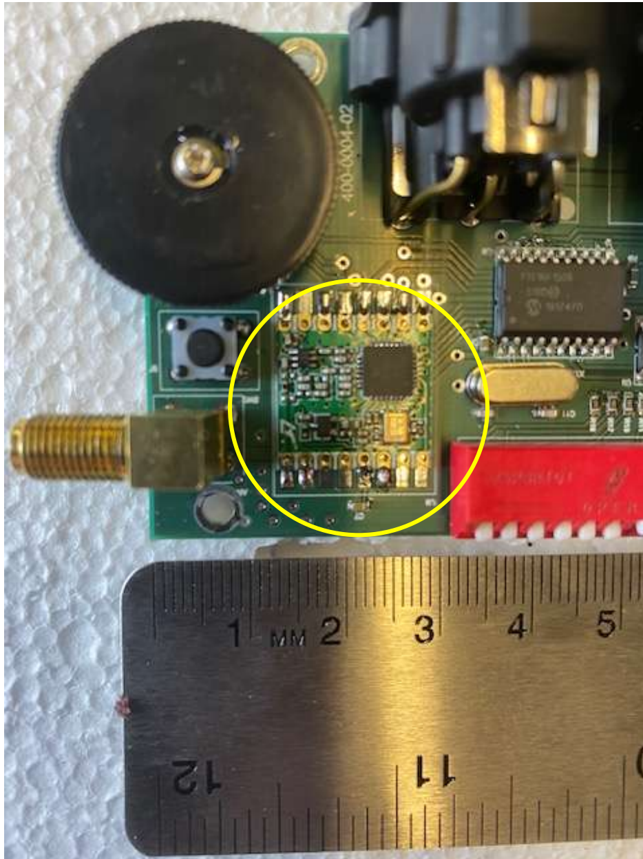
Figure 8. Radio Module
