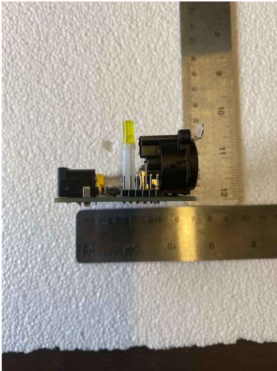
Figure 4. PCB (Back)
