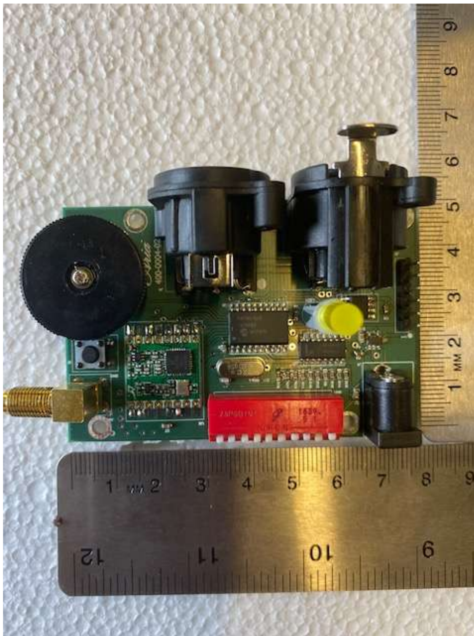
Figure 2. PCB (Top)
