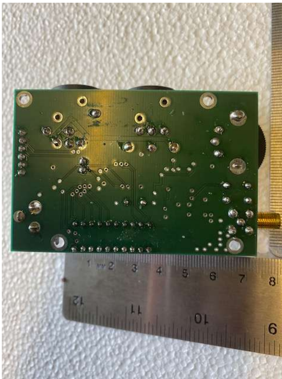
Figure 7. PCB (Bottom)
