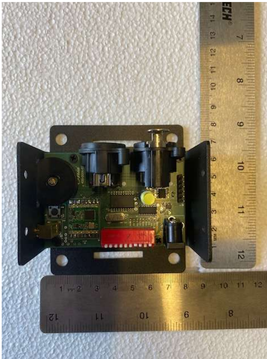
Figure 1. PCB (Mounted)
