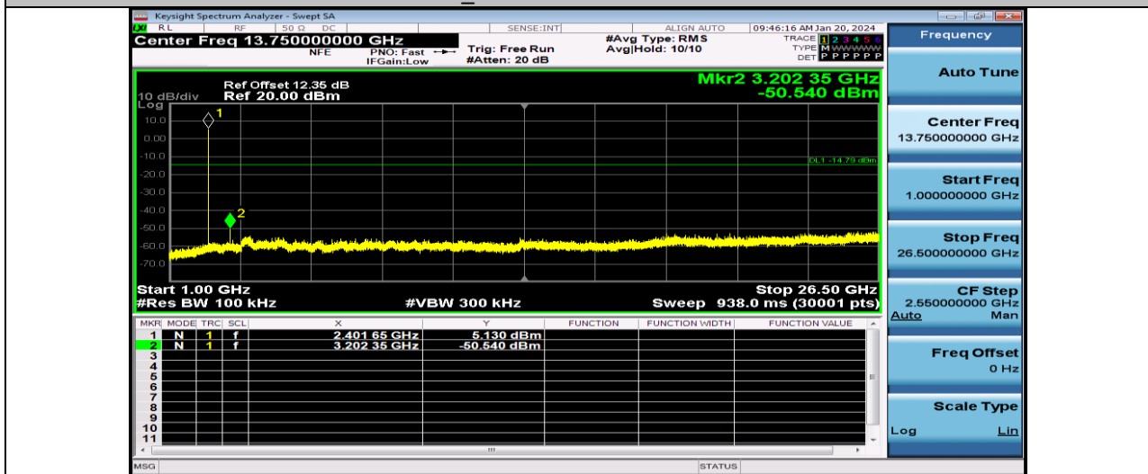
BLE_2M-Ant1-2402-1000~26500
