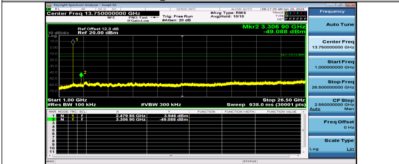
BLE_1M-Ant1-2480-1000~26500
