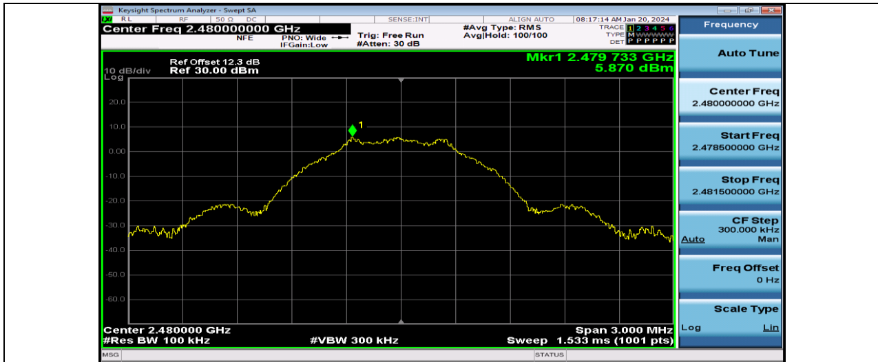
BLE_1M-Ant1-2480-0~Reference
