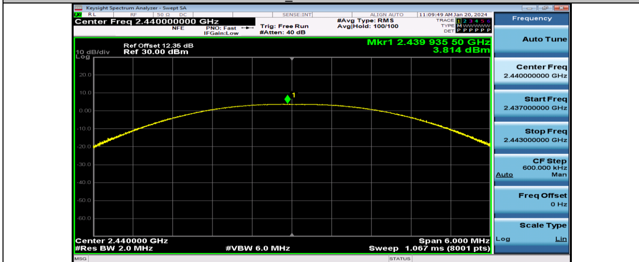
BLE_1M-Ant1-2440
