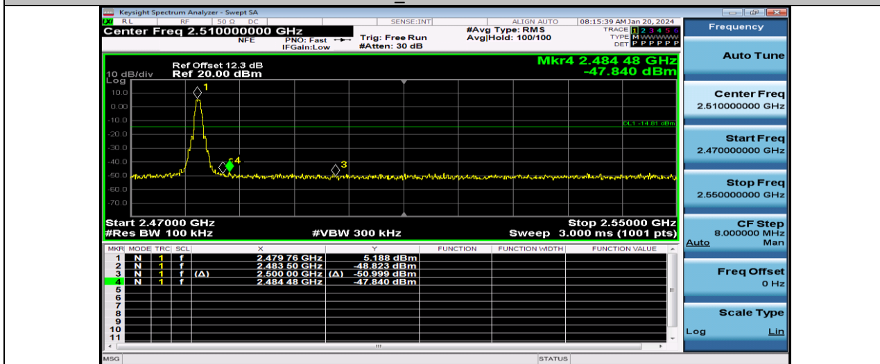
BLE_1M-Ant1-2480
