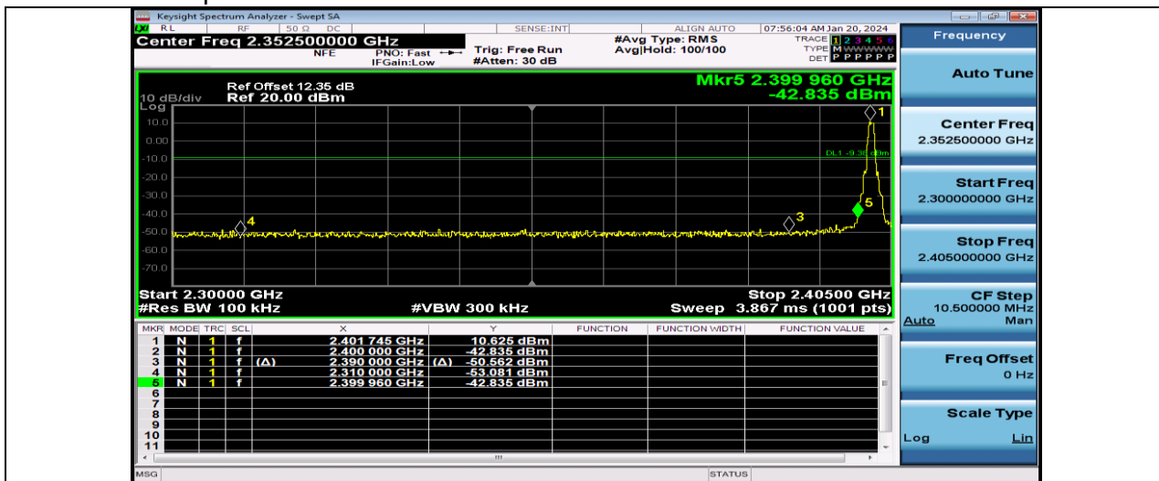
BLE_1M-Ant1-2402
