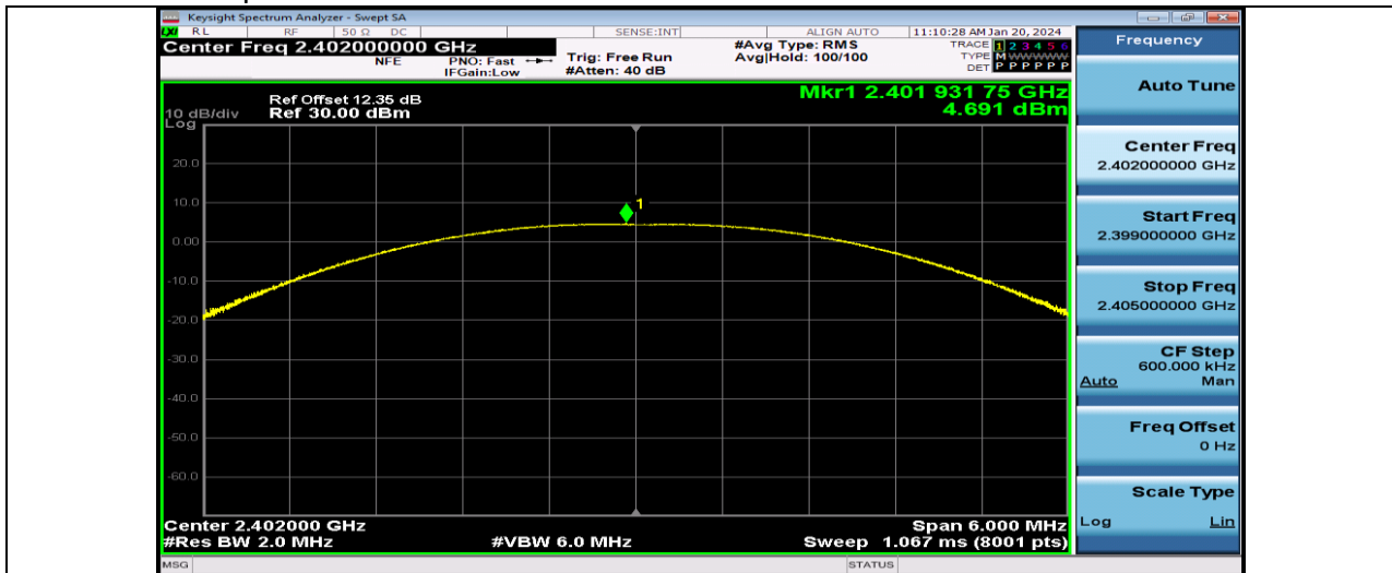
BLE_1M-Ant1-2402
