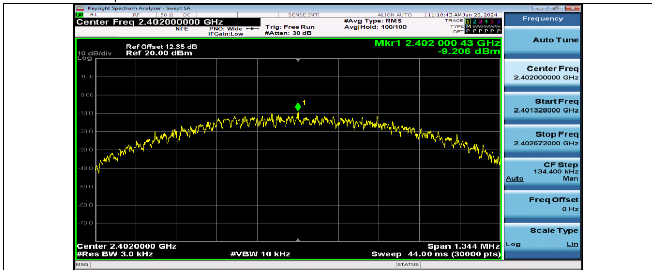
BLE_1M-Ant1-2402
