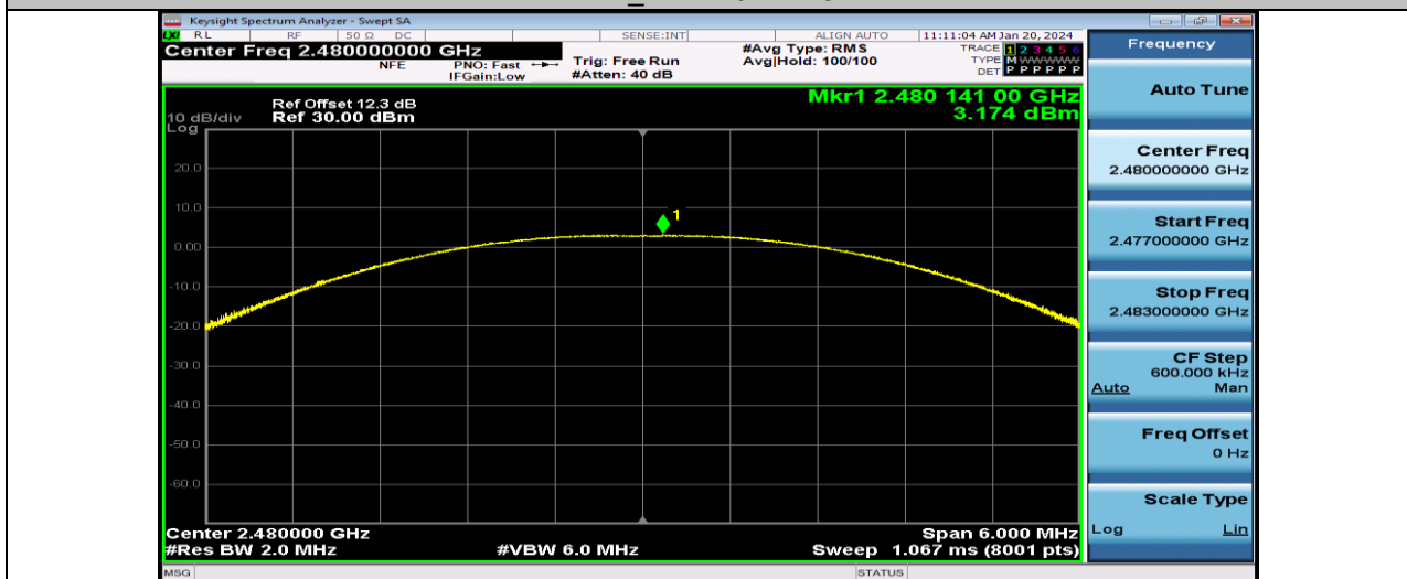
BLE_1M-Ant1-2480
