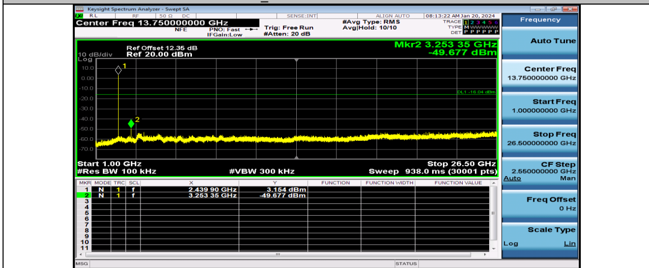
BLE_1M-Ant1-2440-1000~26500
