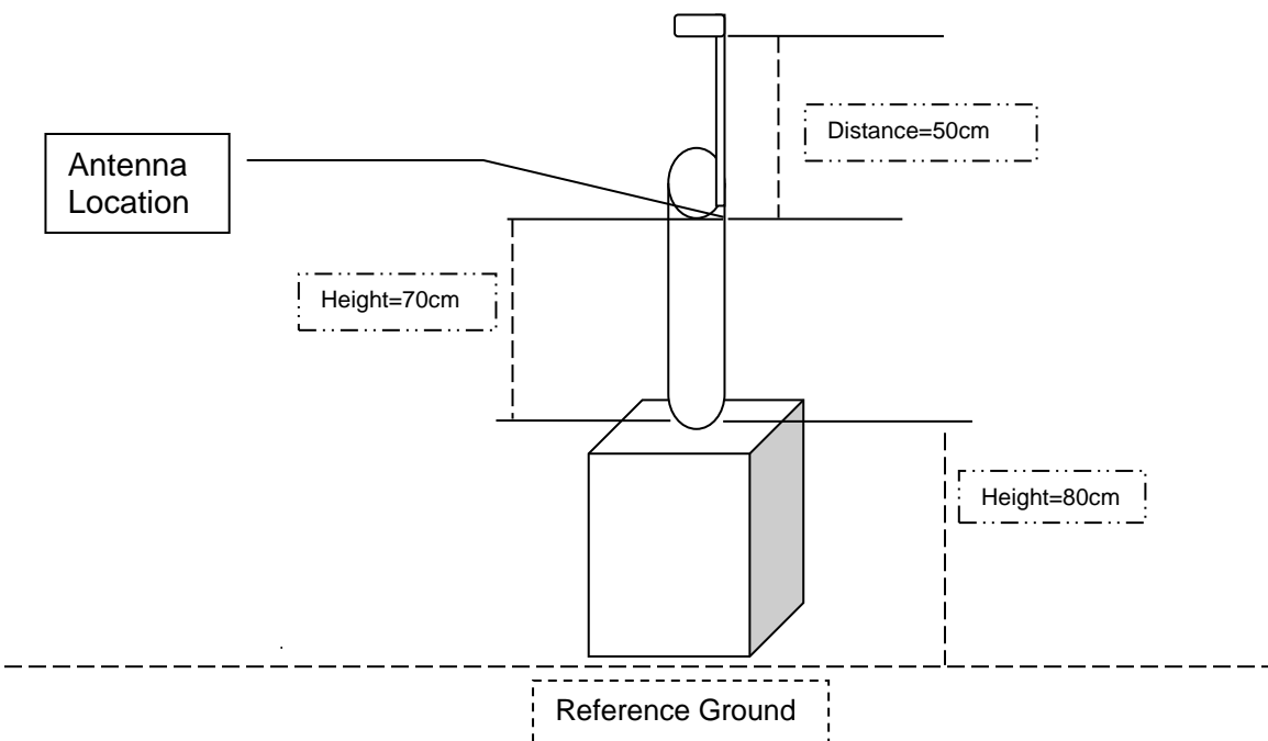
RADIATED RF MEASUREMENT SETUP (ABOVE 1 GHz- Xaxis)-Part 2
