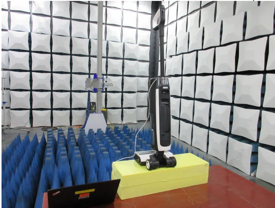
RADIATED RF MEASUREMENT SETUP (ABOVE 1 GHz- X axis) -Part 1
