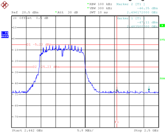
ANT1+ANT2 TX 11n HT20: Band edge-right side
