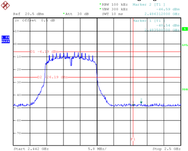
ANT1 TX 11n HT20: Band edge-right side
