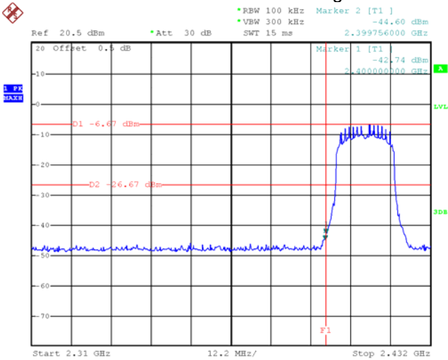
ANT1 TX 11n HT20: Band edge-left side
