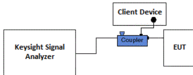
Figure 7-5. Test Instrument & Measurement Setup
