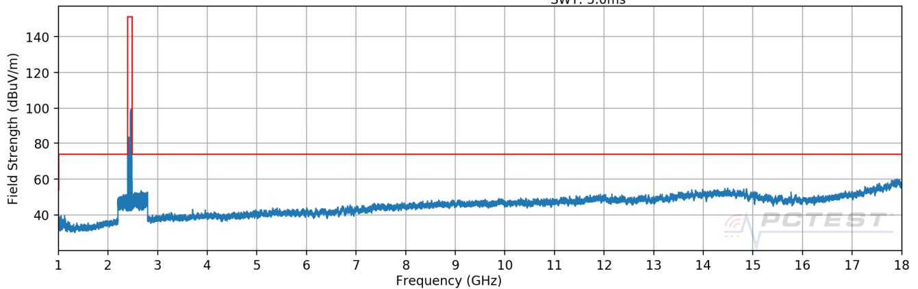
Plot 7-51. Radiated Spurious Plot above 1GHz (802.11b – Ch. 11)
