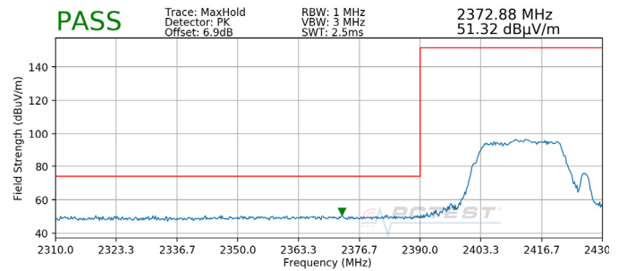
Plot 7-54. Radiated Restricted Lower Band Edge Measurement (Peak)
