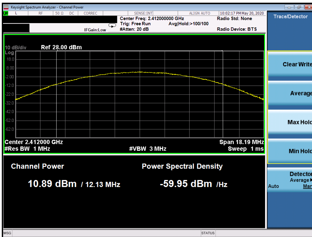
Plot 7-10. Average Conducted Output Power Plot (802.11b – Ch. 1)
