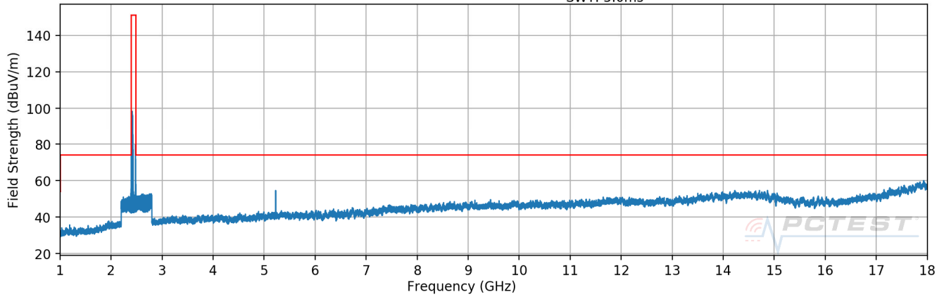
Plot 7-49. Radiated Spurious Plot above 1GHz (802.11b – Ch. 1)
