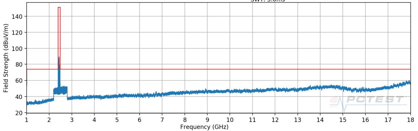
Plot 7-50. Radiated Spurious Plot above 1GHz (802.11b – Ch. 6)
