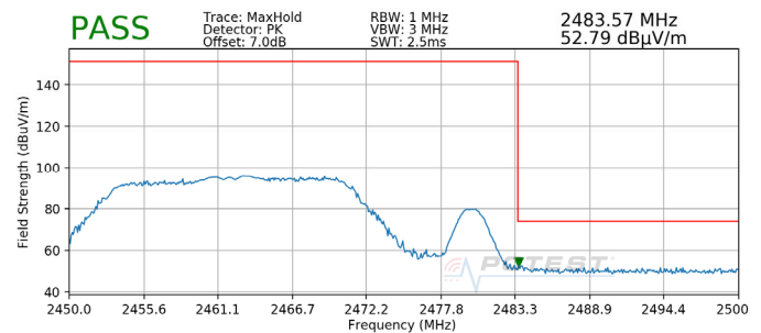
Plot 7-56. Radiated Restricted Upper Band Edge Measurement (Peak)
