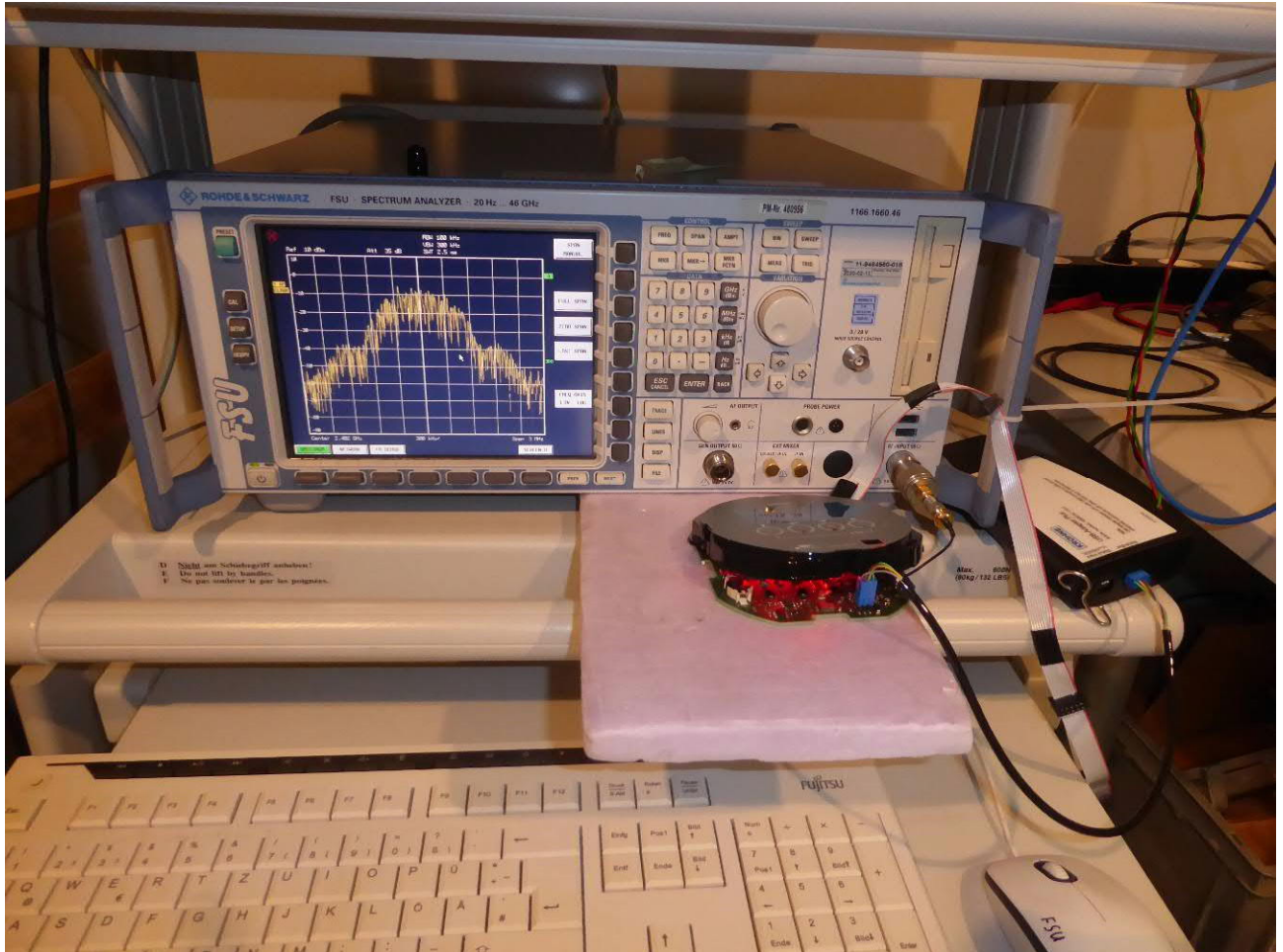
Test setup – conducted measurement at the antenna port
