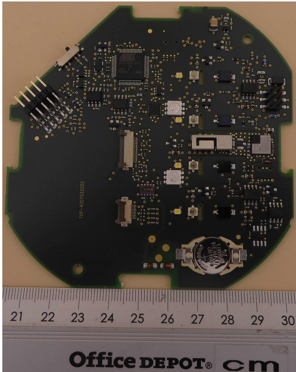
PCB – top view
