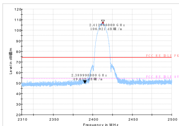
Peak detector
