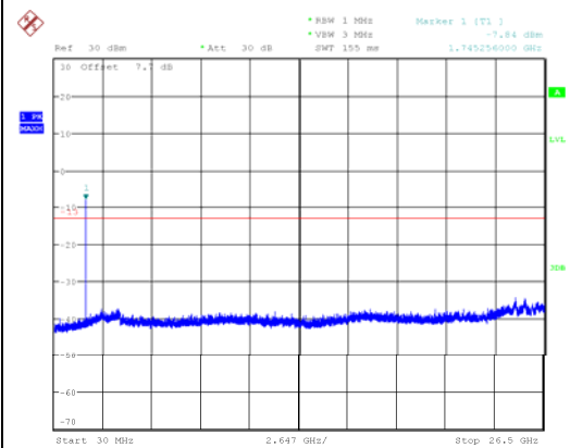
LTE band 66: 30MHz – 26GHz
