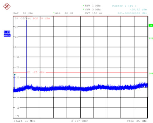
LTE band41: 30MHz – 26GHz
