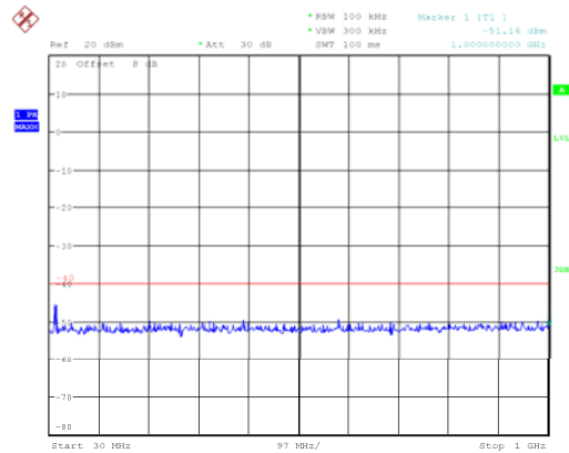
LTE band40(upper): 30MHz – 1GHz
