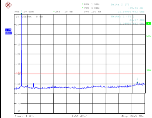
LTE band 40(upper): 1GHz – 26GHz
