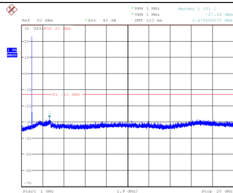
Channel 9538: 1GHz~20GHz
