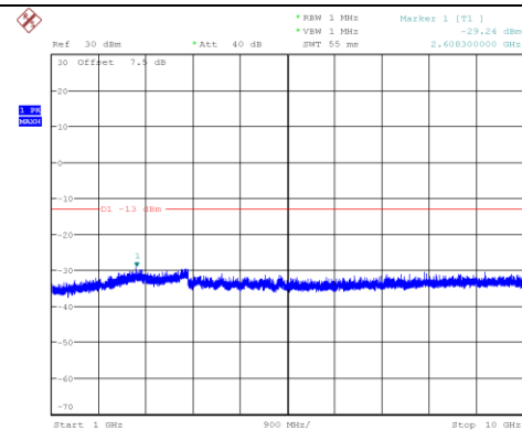
Channel 4175: 1GHz~10GHz
