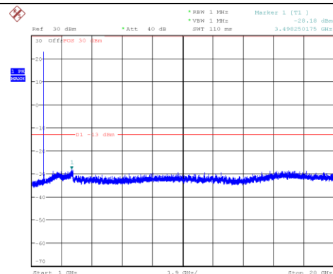
Channel 1312: 1GHz~20GHz
