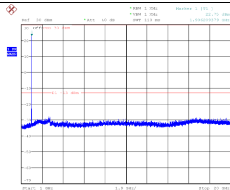
Channel 9262: 1GHz~20GHz
