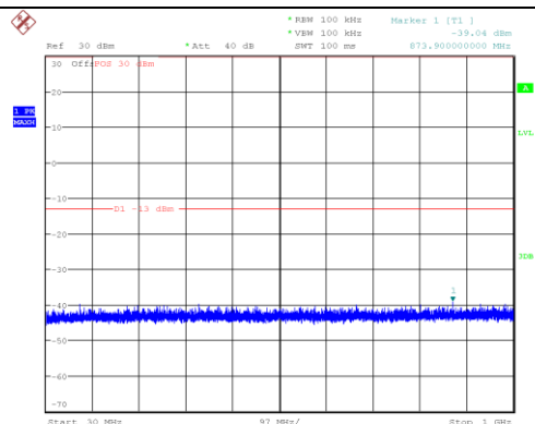
Channel 9400: 30MHz~1GHz
