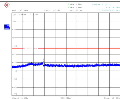
Channel 4232: 1GHz~10GHz
