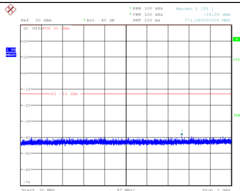
Channel 1312: 30MHz~1GHz
