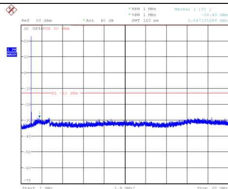
Channel 9400: 1GHz~20GHz
