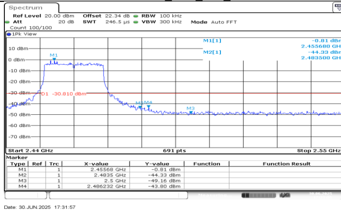
11AX20SISO_Ant1_High_2462
