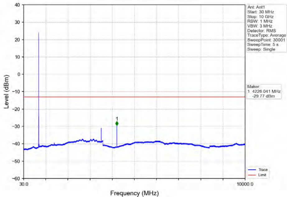
Band17_5MHz_QPSK_LCH_706.5MHz_RB_25_0_NTNV
