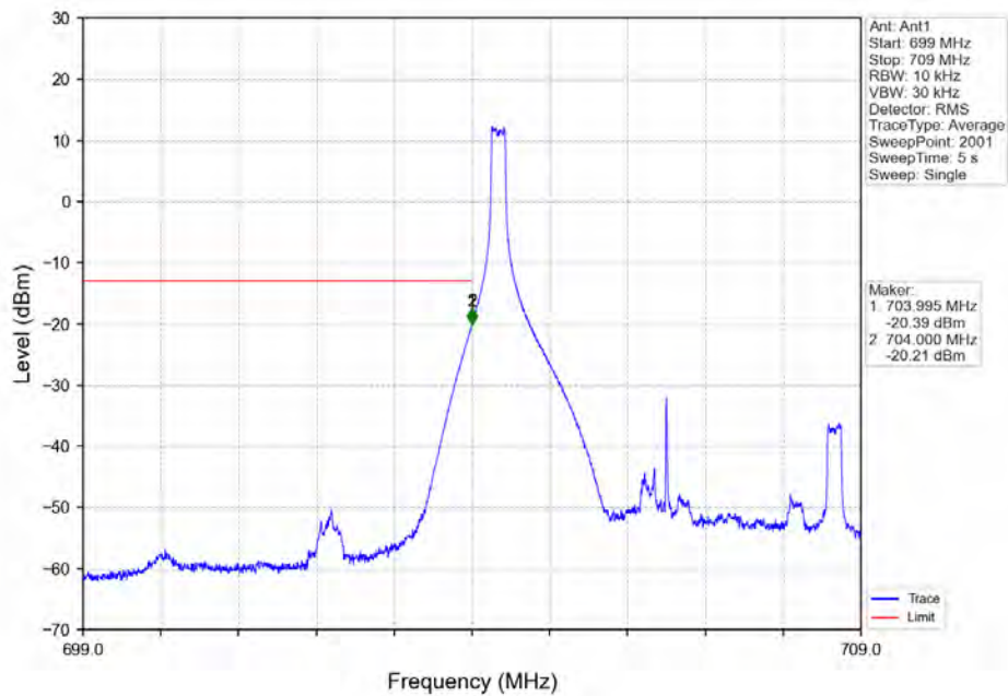
Band17_5MHz_QPSK_LCH_706.5MHz_RB_1_0_NTNV
