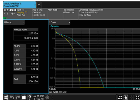
N25(20M)_DFT-s- OFDM_QPSK_Outer_Full_Mid_CH
