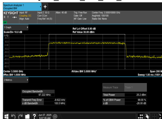
N77(100M)_CP-OFDM_16 QAM_Outer_Full_Mid_CH
