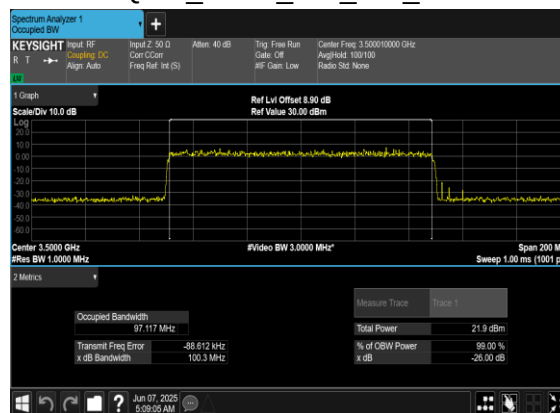
N77(100M)_CP-OFDM_256 QAM_Outer_Full_Mid_CH
