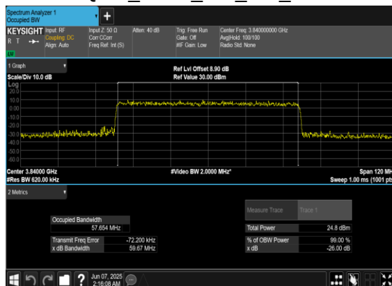
N77(60M)_CP-OFDM_16 QAM_Outer_Full_Mid_CH
