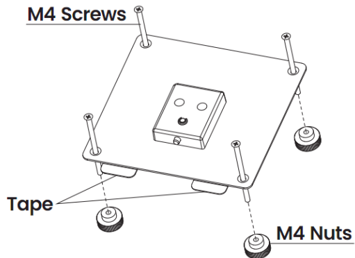
Figure 7:installation 1
