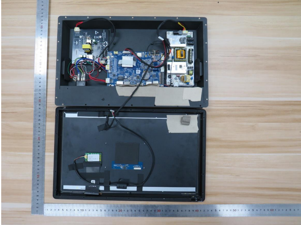
Model: K20 Internal View of EUT-1
