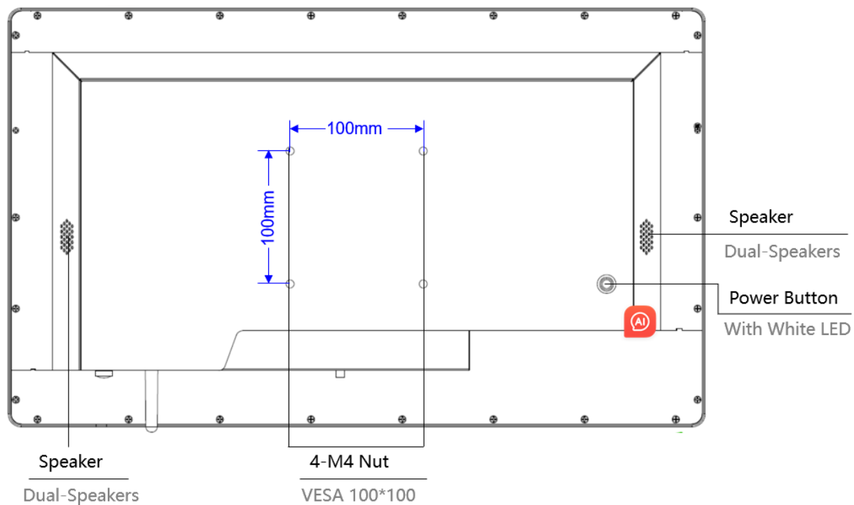
Figure 2: Back view
