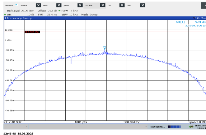
Figure 7.6-: PSD on high channel, 2Mbps
