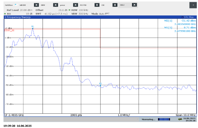
Figure 7.7-15: Conducted band edge spurious emissions at 2483.5 MHz, 2Mbps
