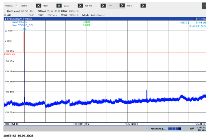
Figure 7.7-9: Conducted spurious emissions on high channel, 1Mbps
