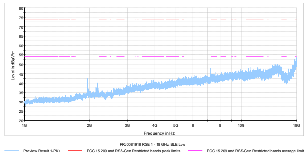
Figure 7.7-21: Radiated spurious emissions on Low channel, 1 – 18 GHz
