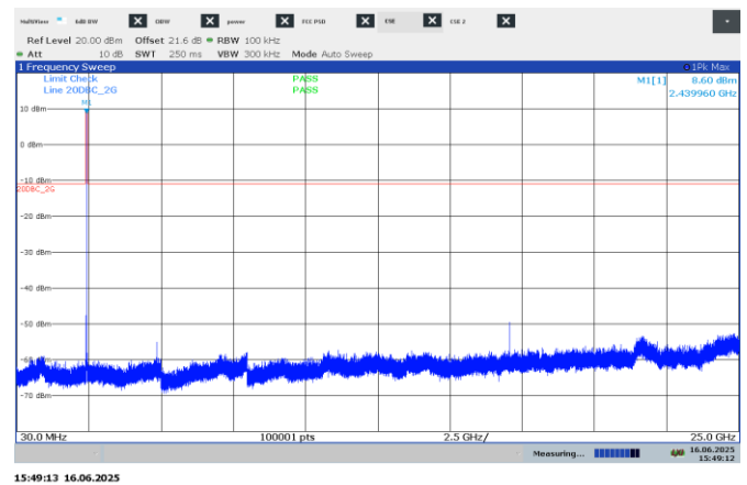
Figure 7.7-8: Conducted spurious emissions on mid channel, 1Mbps
