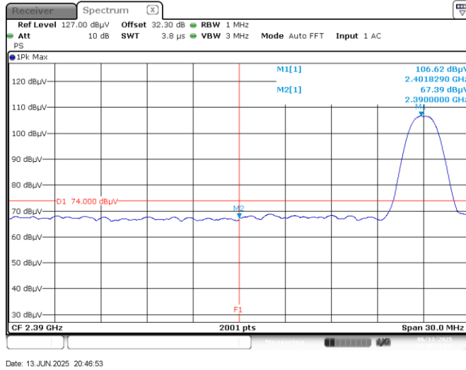
Figure 7.7-1: Restricted band edge spurious emissions at 2390 MHz, Peak, 1Mbps
