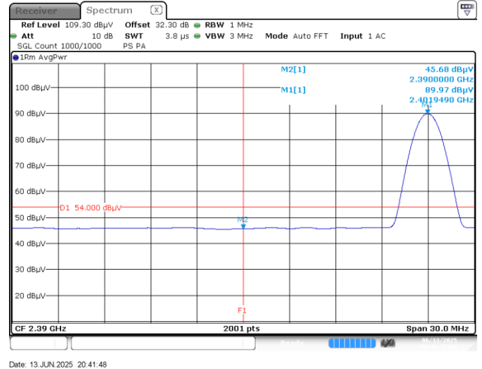
Figure 7.7-2: Restricted band edge spurious emissions at 2390 MHz, Average, 1Mbps
