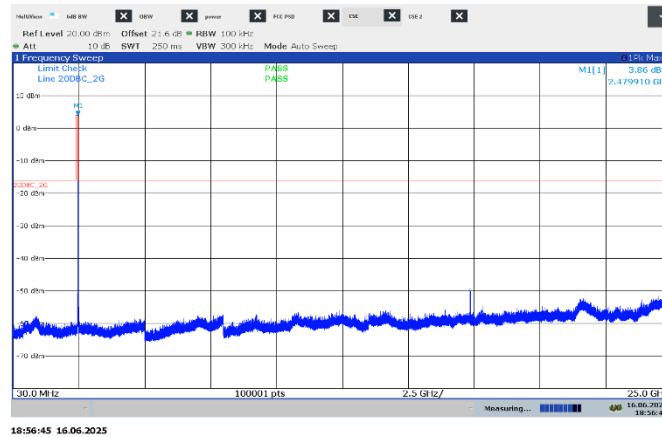
Figure 7.7-18: Conducted spurious emissions on high channel, 2Mbps
