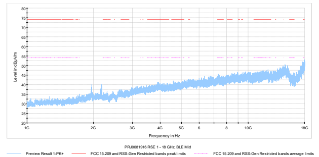
Figure 7.7-22: Radiated spurious emissions on Mid channel, 1 – 18 GHz
