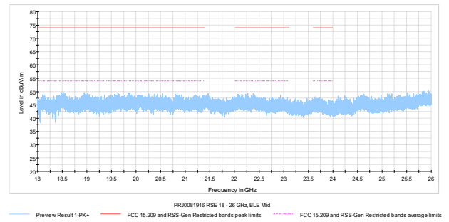
Figure 7.7-24: Radiated spurious emissions on Mid channel, 18 – 26 GHz
