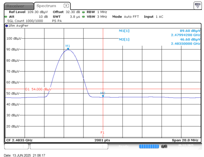
Figure 7.7-4: Restricted band edge spurious emissions at 2483.5 MHz, Average, 1Mbps
