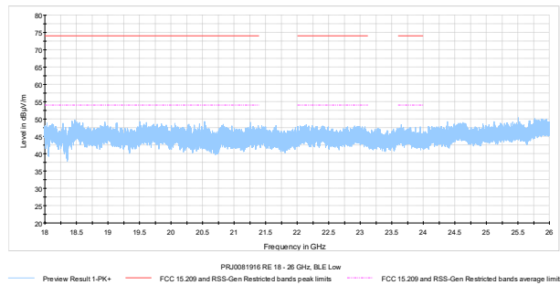
Figure 7.7-23: Radiated spurious emissions on Low channel, 18 – 26 GHz
