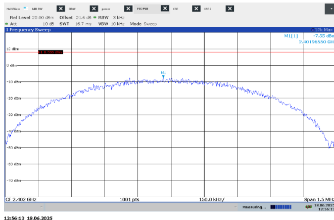
Figure 7.8-1: PSD on low channel, 1Mbps
