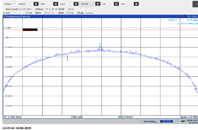
Figure 7.4-: PSD on low channel, 2Mbps
