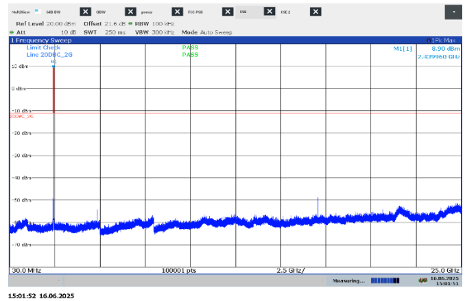
Figure 7.7-17: Conducted spurious emissions on mid channel, 2Mbps
