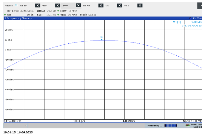
Figure 7.6-3: Output power on high channel, 1Mbps
