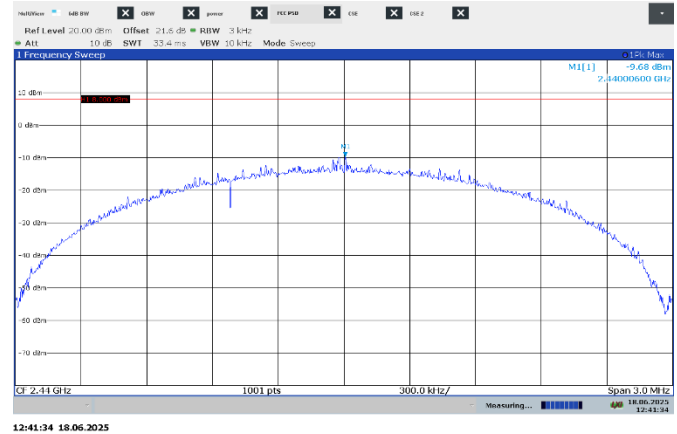
Figure 7.5-: PSD on mid channel, 2Mbps
