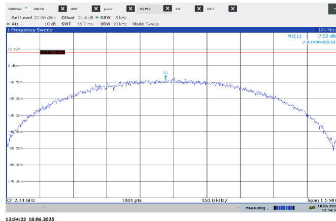
Figure 7.8-2: PSD on mid channel, 1Mbps
