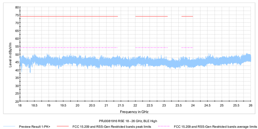
Figure 7.7-27: Radiated spurious emissions on high channel, 18 – 26 GHz
