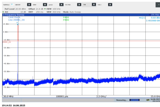
Figure 7.7-7: Conducted spurious emissions on low channel, 1Mbps
