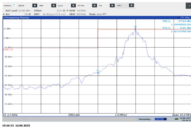
Figure 7.7-5: Conducted band edge spurious emissions at 2400 MHz, 1Mbps
