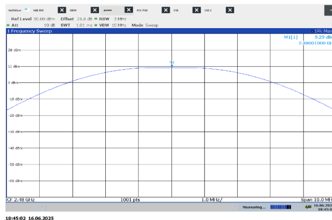
Figure 7.6-6: Output power on high channel, 2Mbps
