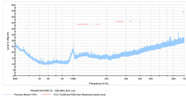
Figure 7.7-19: Radiated spurious emissions on Low channel, 30 – 1000 MHz
