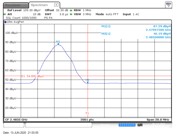
Figure 7.7-13: Restricted band edge spurious emissions at 2483.5 MHz, Average, 2Mbps
