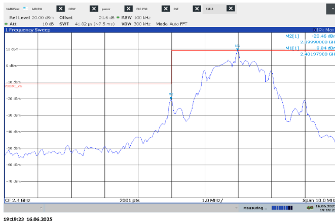
Figure 7.7-14: Conducted band edge spurious emissions at 2400 MHz, 2Mbps
