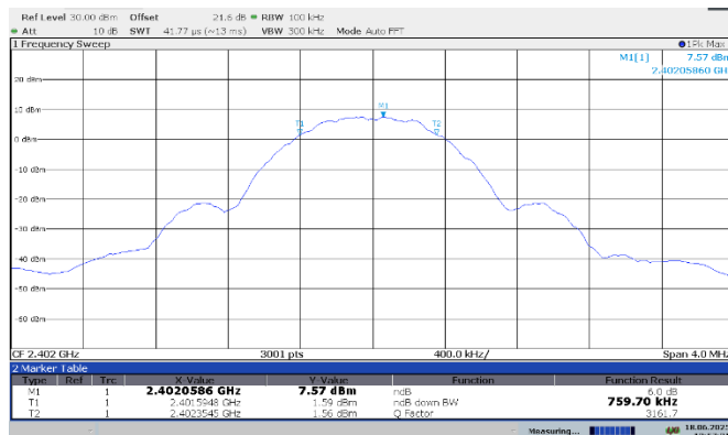
Figure 7.4-1: 6 dB bandwidth – 1Mbps, sample plot
