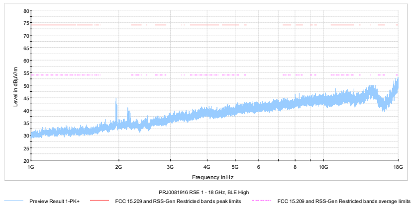
Figure 7.7-26: Radiated spurious emissions on high channel, 1 – 18 GHz
