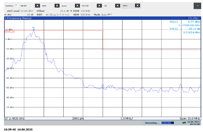
Figure 7.7-6: Conducted band edge spurious emissions at 2483.5 MHz, 1Mbps
