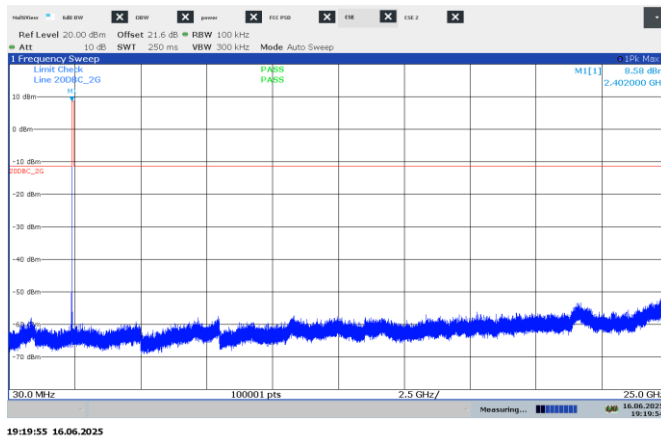
Figure 7.7-16: Conducted spurious emissions on low channel, 2Mbps
