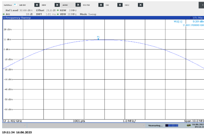
Figure 7.6-1: Output power on low channel, 1Mbps
