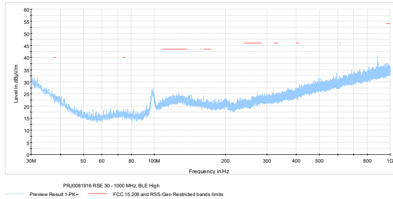
Figure 7.7-25: Radiated spurious emissions on high channel, 30 – 1000 MHz
