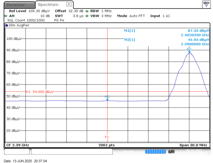
Figure 7.7-11: Restricted band edge spurious emissions at 2390 MHz, Average, 2Mbps
