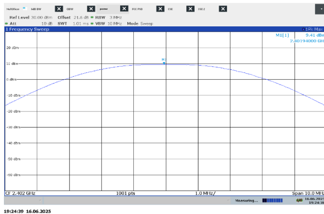
Figure 7.6-4: Output power on low channel, 2Mbps
