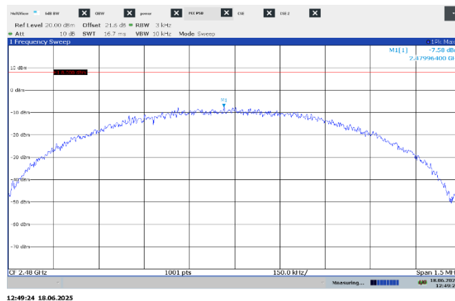
Figure 7.8-3: PSD on high channel, 1Mbps
