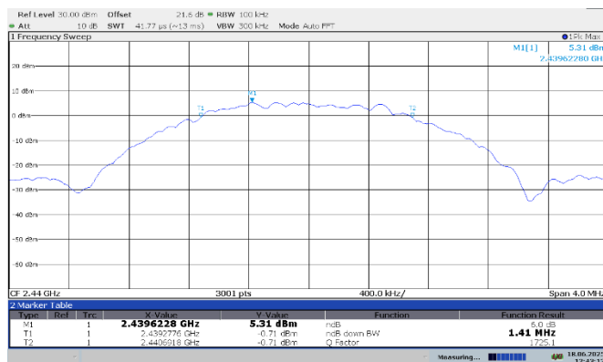
Figure 7.4-3: 6 dB bandwidth – 2Mbps, sample plot
