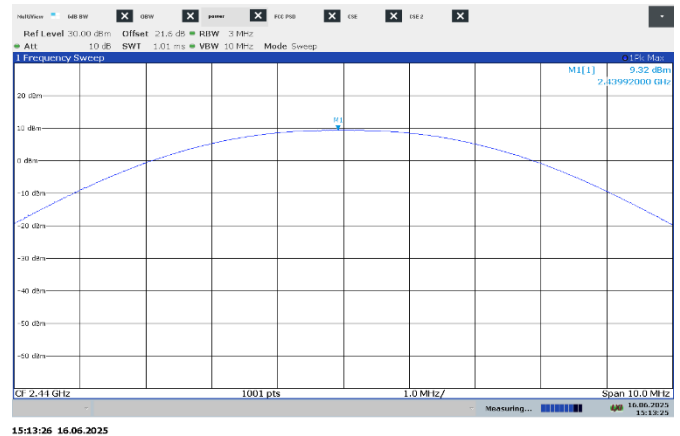
Figure 7.6-2: Output power on mid channel, 1Mbps
