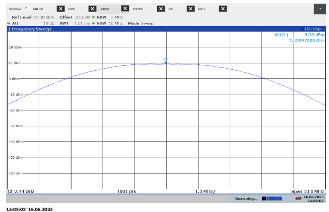
Figure 7.6-5: Output power on mid channel, 2Mbps
