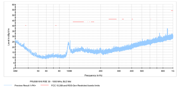
Figure 7.7-20: Radiated spurious emissions on Mid channel, 30 – 1000 MHz
