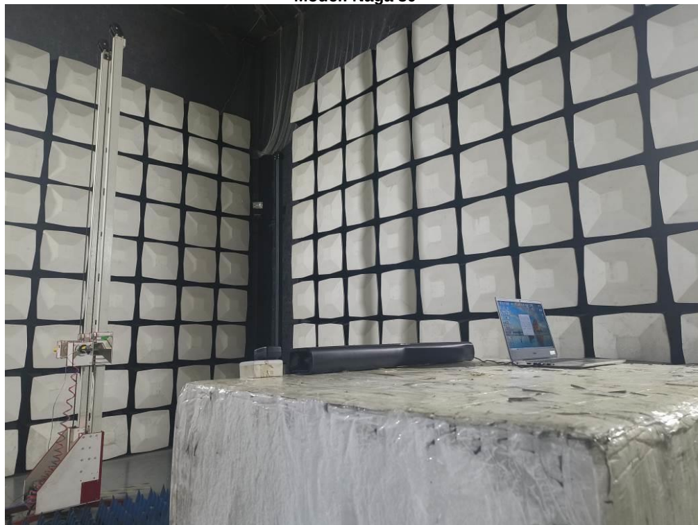
Radiated emission (Above 1000MHz) Model: Naga 80
